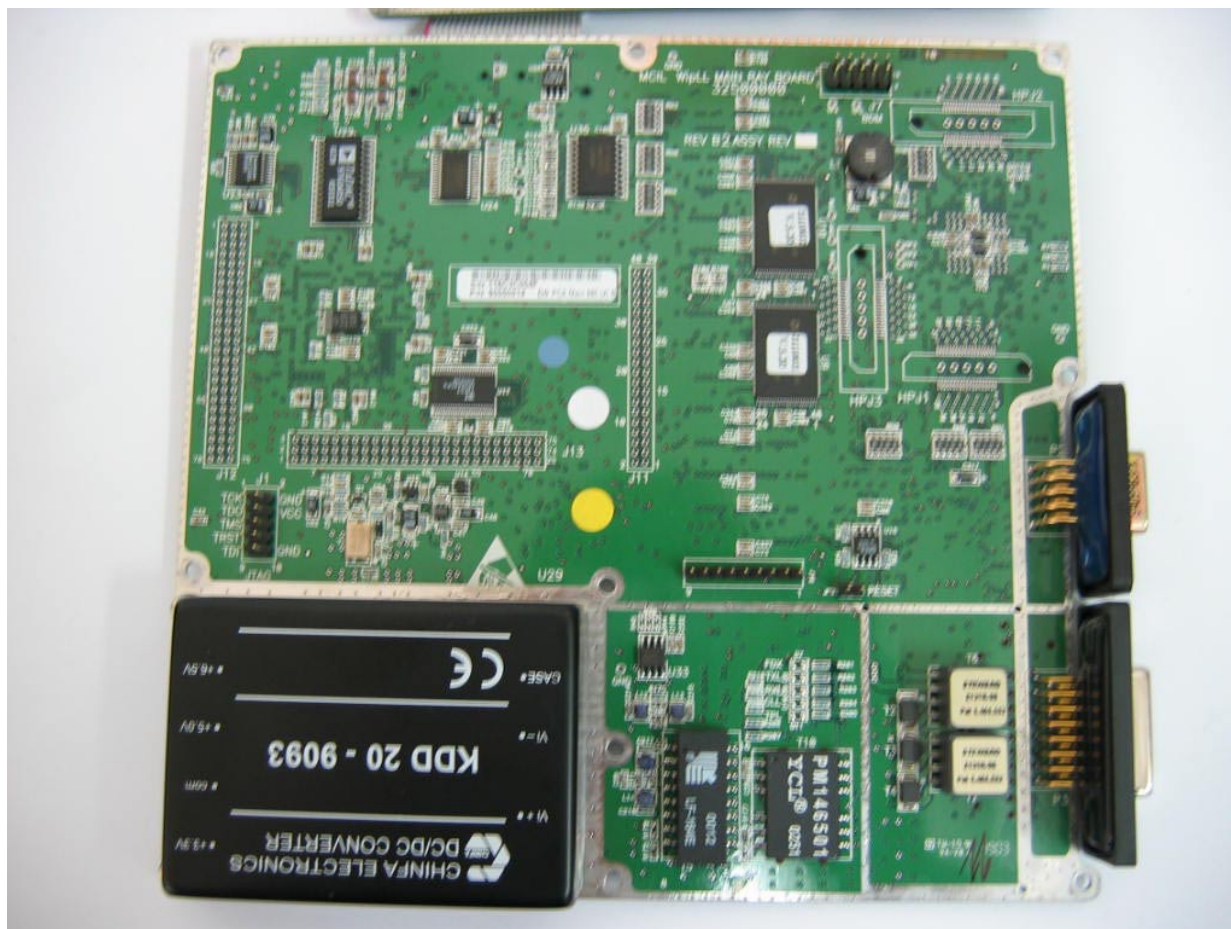
Photograph No.5 BSR 700MHz, digital board front view
