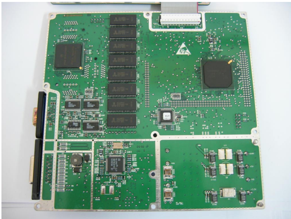
Photograph No.6 BSR 700MHz, digital board second side view
