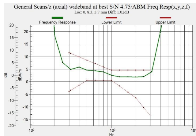
Figure C.18 Frequency Response of W1900 - OTT VoIP
