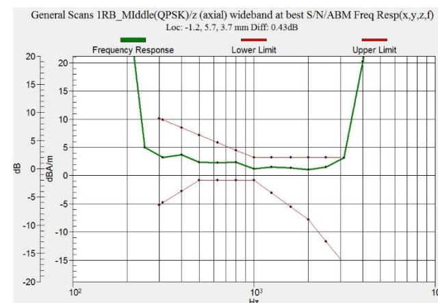
Figure C.15 Frequency Response of LTE B41 Power Class 3
