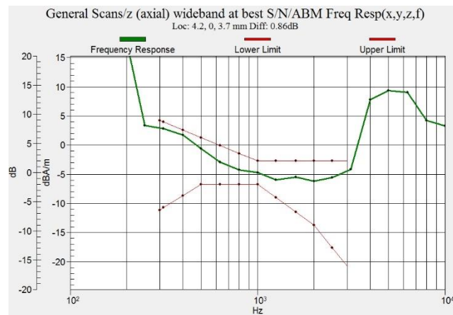
Figure C.17 Frequency Response of EDGE 1900 - OTT VoIP
