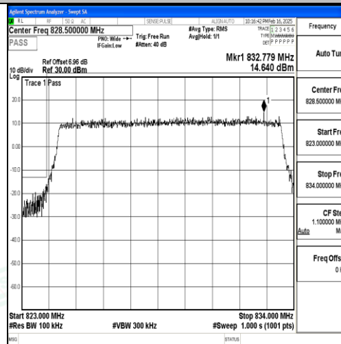
Band5_10MHz_16QAM_20450_50RB#0
