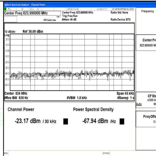
Band5_3MHz_16QAM_20415_15RB#0_Final1
