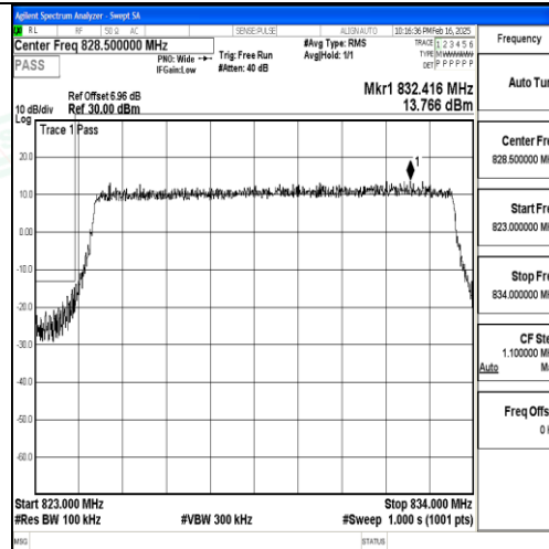
Band5_10MHz_QPSK_20450_50RB#0
