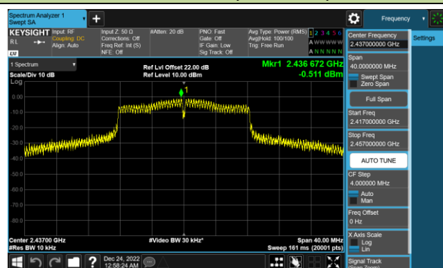
Channel 06 (2437MHz)
