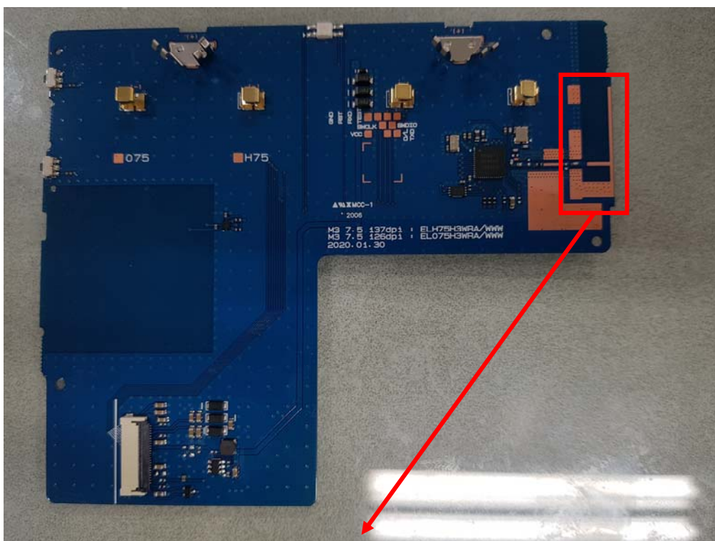
Transmission Antenna(BLE)
