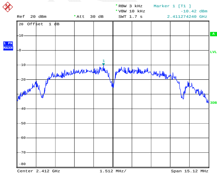
Power Spectral Density, 802.11b Low Channel, Chain 0
