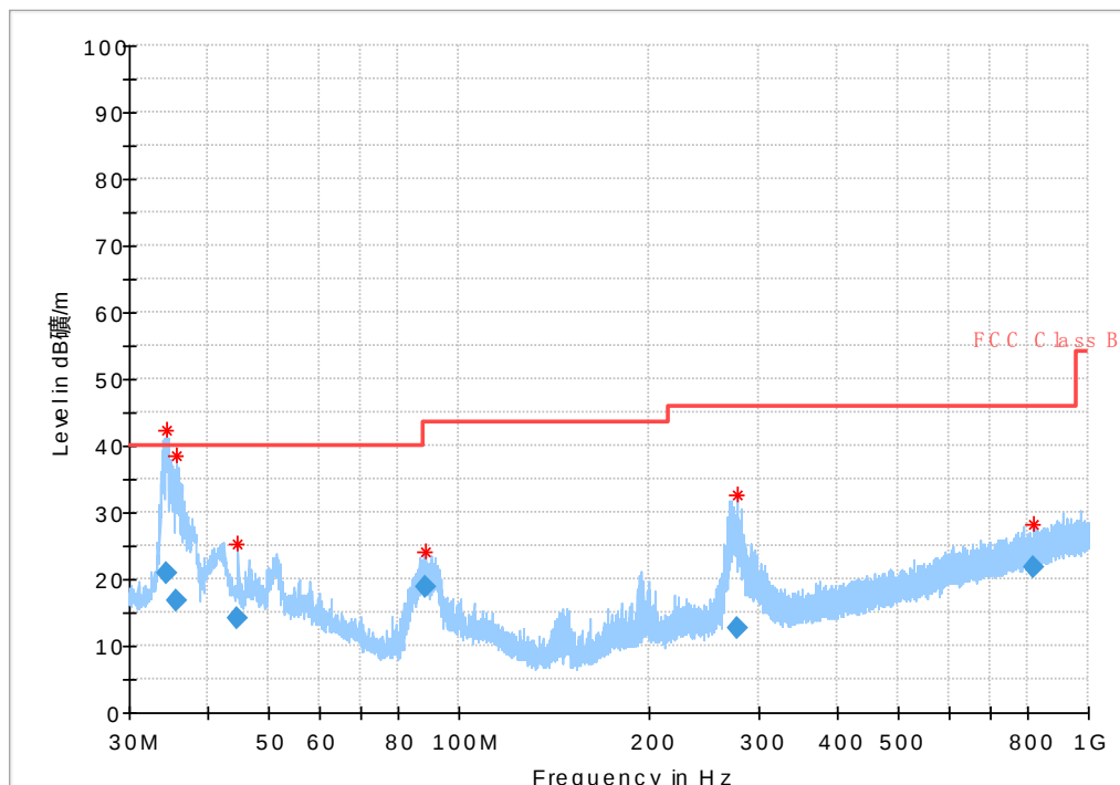
Fig. 49 Radiated Spurious Emission (802.11n-HT40, ch38, 30 MHz-1 GHz)
