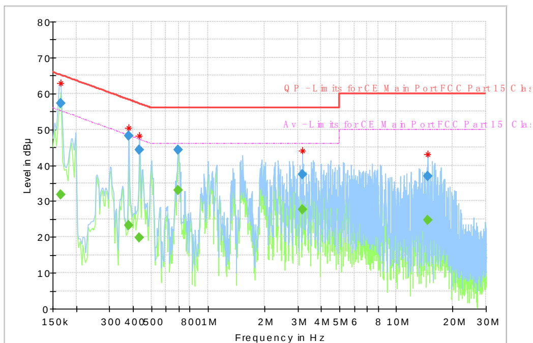
Fig. 60 Conducted Emission(802.11a, TX)
