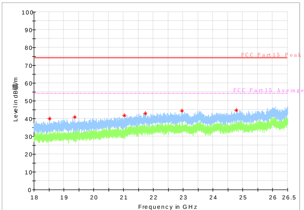
Fig. 58 Radiated Spurious Emission (802.11n-HT40, ch38, 18 GHz-26.5 GHz)
