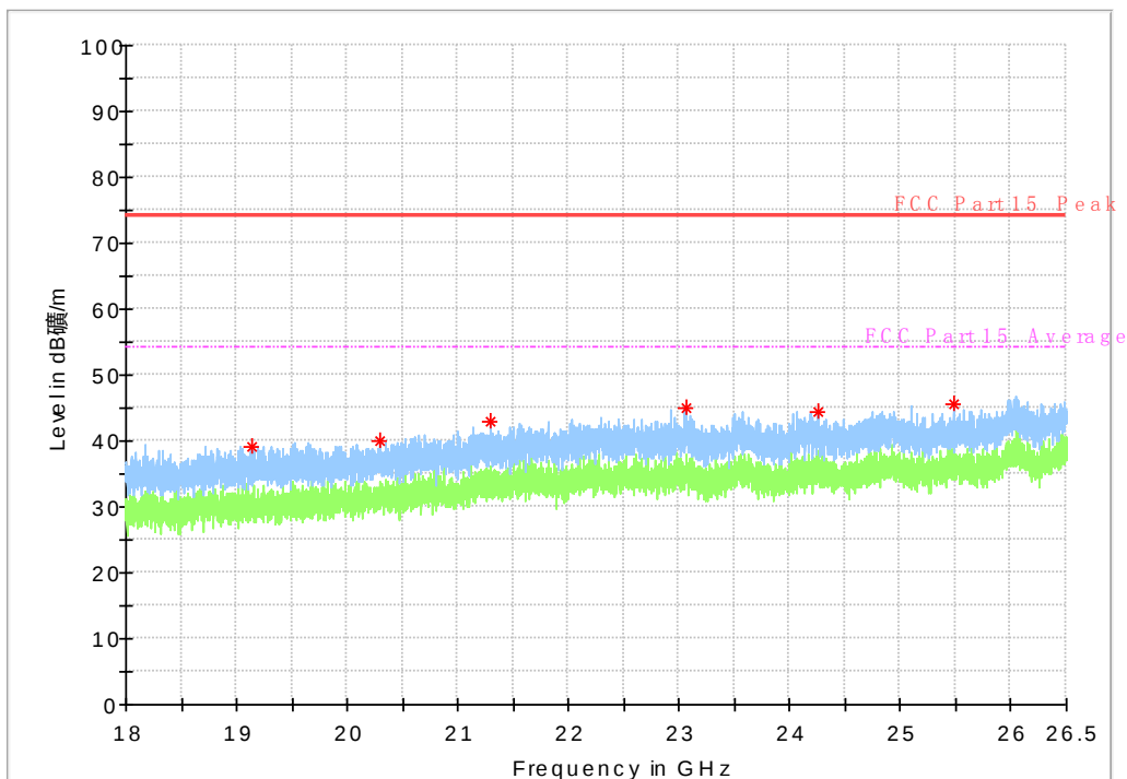
Fig. 47 Radiated Spurious Emission (802.11n-HT20, ch36, 18 GHz-26.5 GHz)
