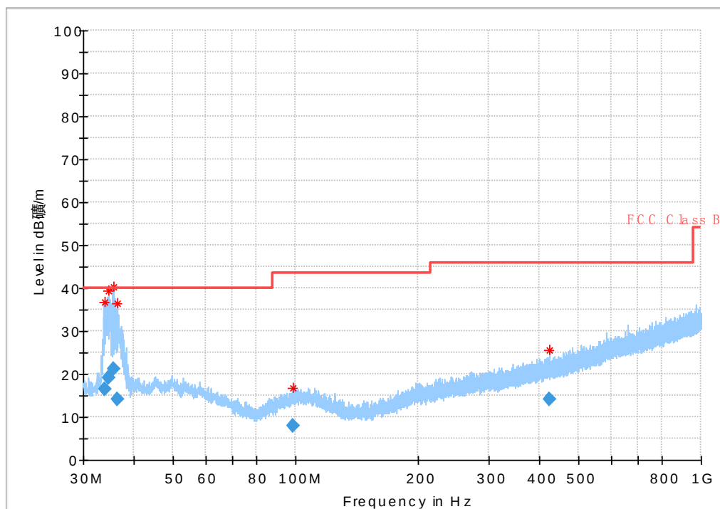
Fig. 55 Radiated Spurious Emission (802.11n-HT40, ch38, 30 MHz-1 GHz)
