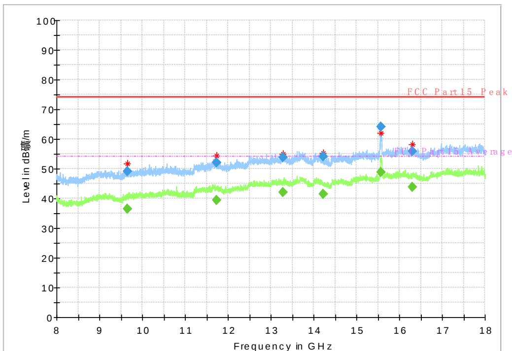
Fig. 51 Radiated Spurious Emission (802.11n-HT40, ch38, 8 GHz-18 GHz)
