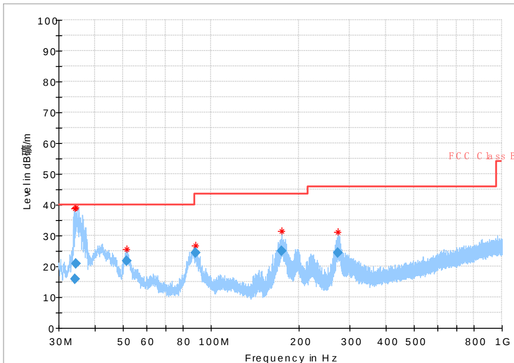
Fig. 39 Radiated Spurious Emission (802.11a, ch36, 30 MHz-1 GHz)
