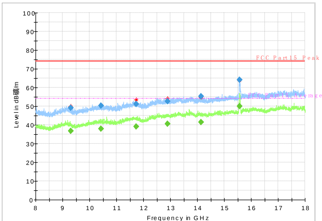
Fig. 57 Radiated Spurious Emission (802.11n-HT40, ch38, 8 GHz-18 GHz)
