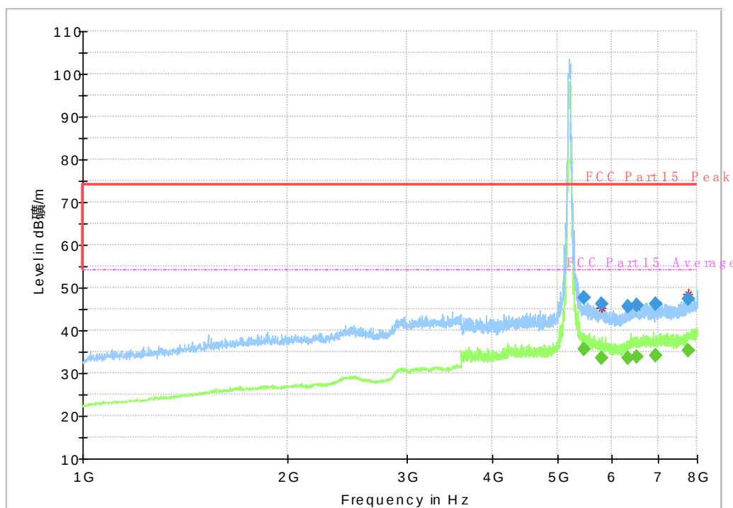
Fig. 56 Radiated Spurious Emission (802.11n-HT40, ch38, 1 GHz-8 GHz)
