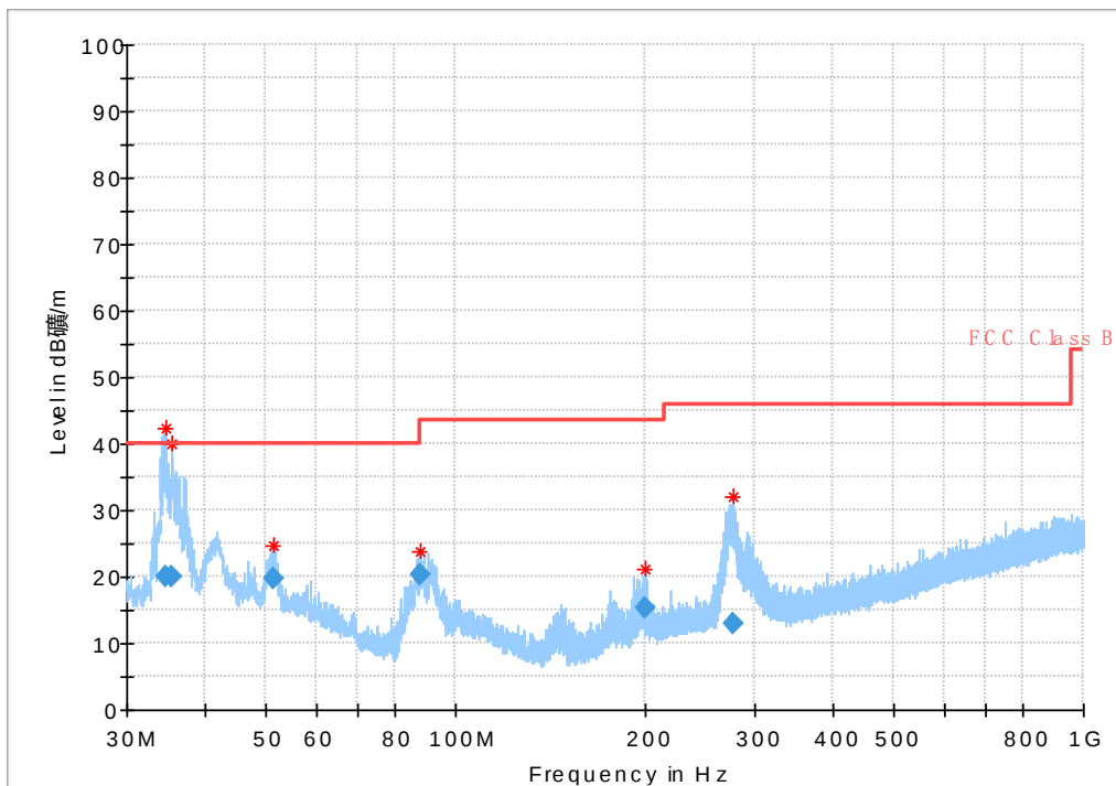
Fig. 44 Radiated Spurious Emission (802.11n-HT20, ch36, 30 MHz-1 GHz)
