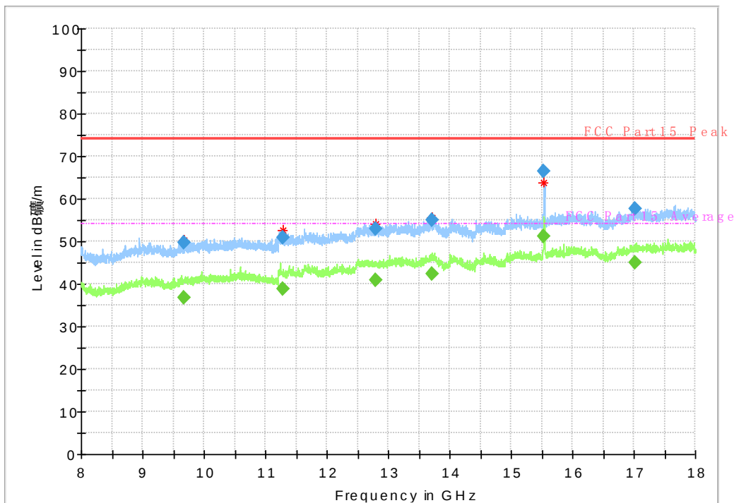
Fig. 46 Radiated Spurious Emission (802.11n-HT20, ch36, 8 GHz-18 GHz)
