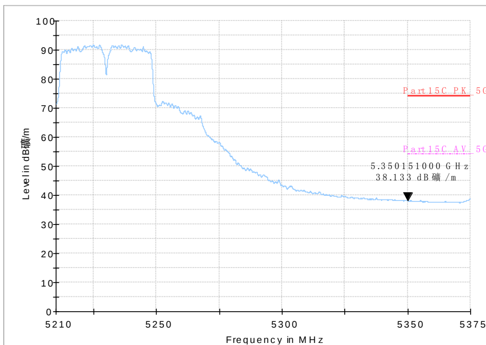
Fig. 38 Band Edges (802.11n-HT40, 5230MHz)
