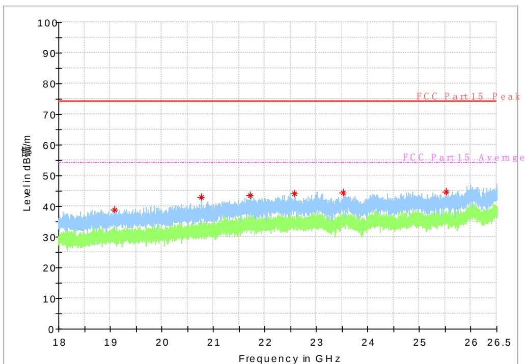
Fig. 52 Radiated Spurious Emission (802.11n-HT40, ch38, 18 GHz-26.5 GHz)
