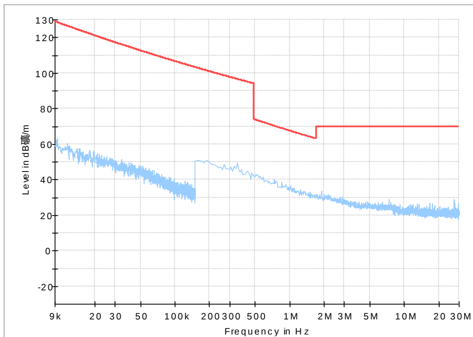
Fig. 54 Radiated Spurious Emission (9kHz-30MHz)
