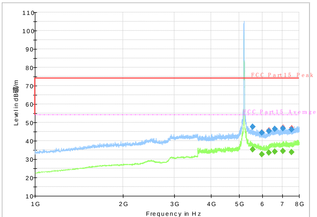
Fig. 40 Radiated Spurious Emission (802.11a, ch36, 1 GHz-8 GHz)
