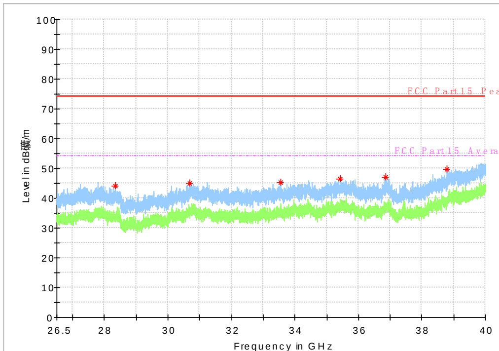
Fig. 43 Radiated Spurious Emission (802.11a, ch36, 26.5 GHz-40 GHz)
