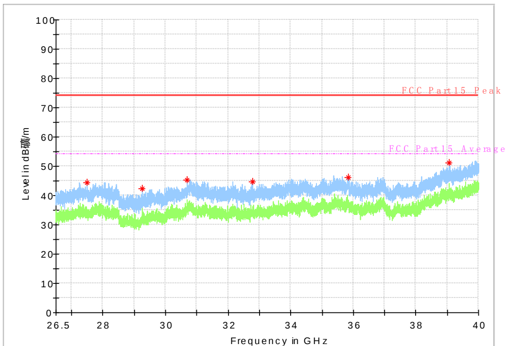
Fig. 48 Radiated Spurious Emission (802.11n-HT20, ch36, 26.5 GHz-40 GHz)
