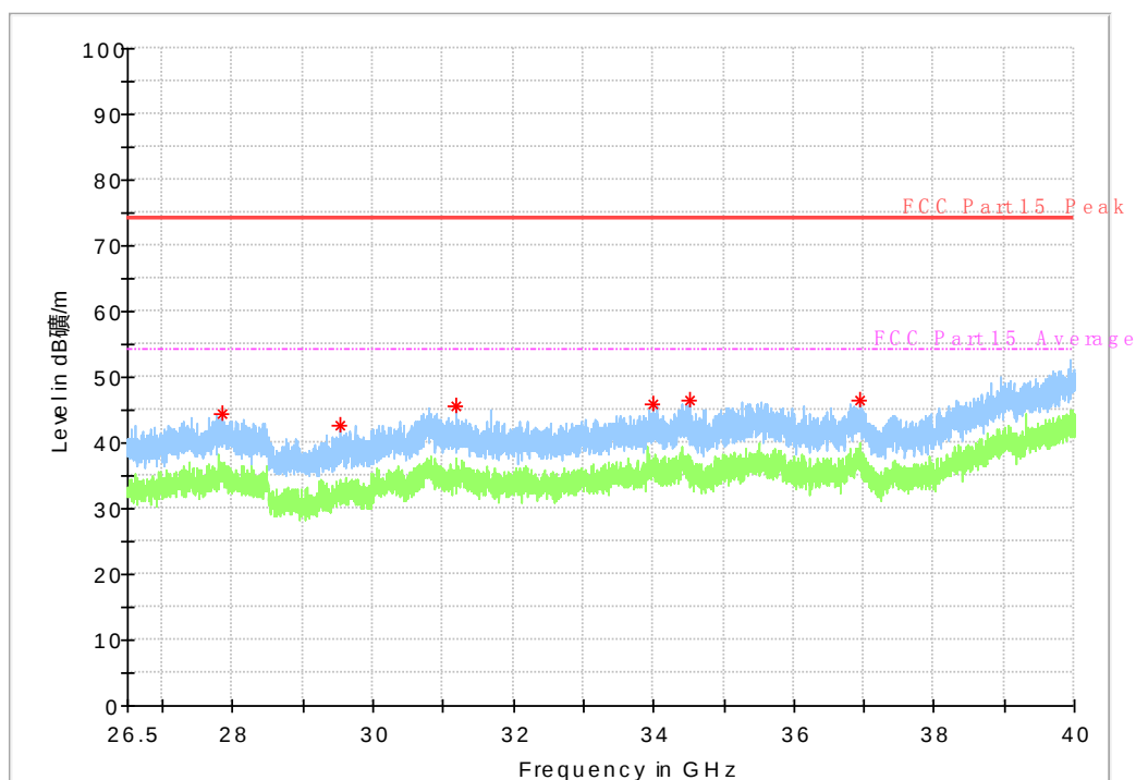
Fig. 59 Radiated Spurious Emission (802.11n-HT40, ch38, 26.5 GHz-40 GHz)
