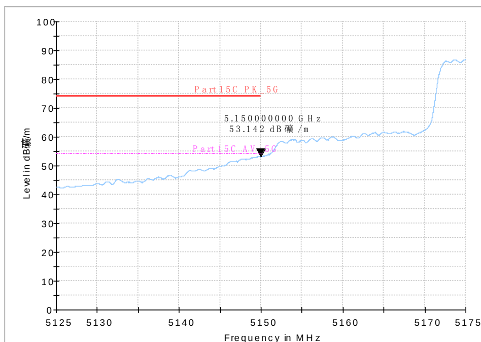
Fig. 37 Band Edges (802.11n-HT40, 5190MHz)
