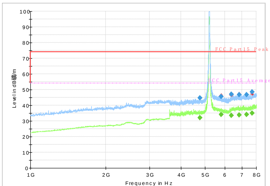
Fig. 50 Radiated Spurious Emission (802.11n-HT40, ch38, 1 GHz-8 GHz)
