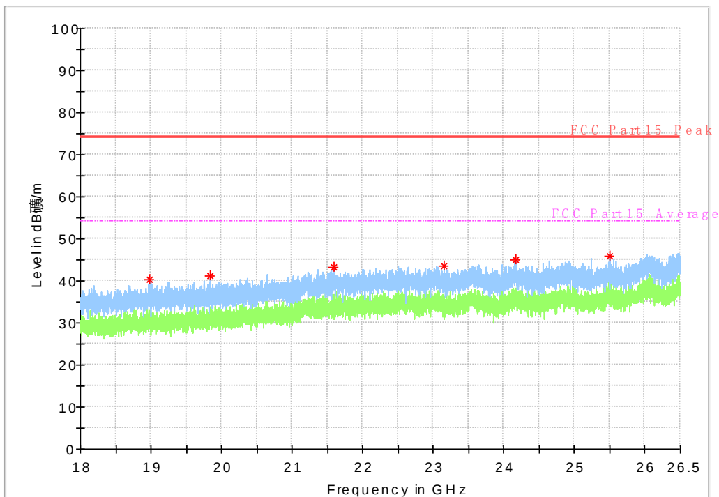
Fig. 42 Radiated Spurious Emission (802.11a, ch36, 18 GHz-26.5 GHz)
