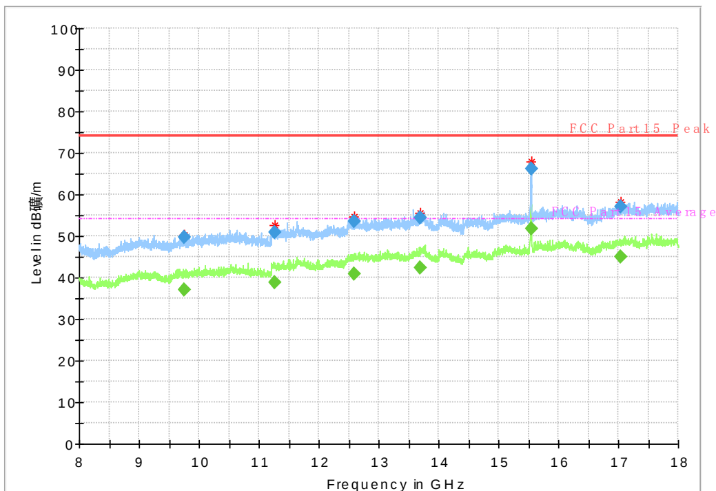
Fig. 41 Radiated Spurious Emission (802.11a, ch36, 8 GHz-18 GHz)
