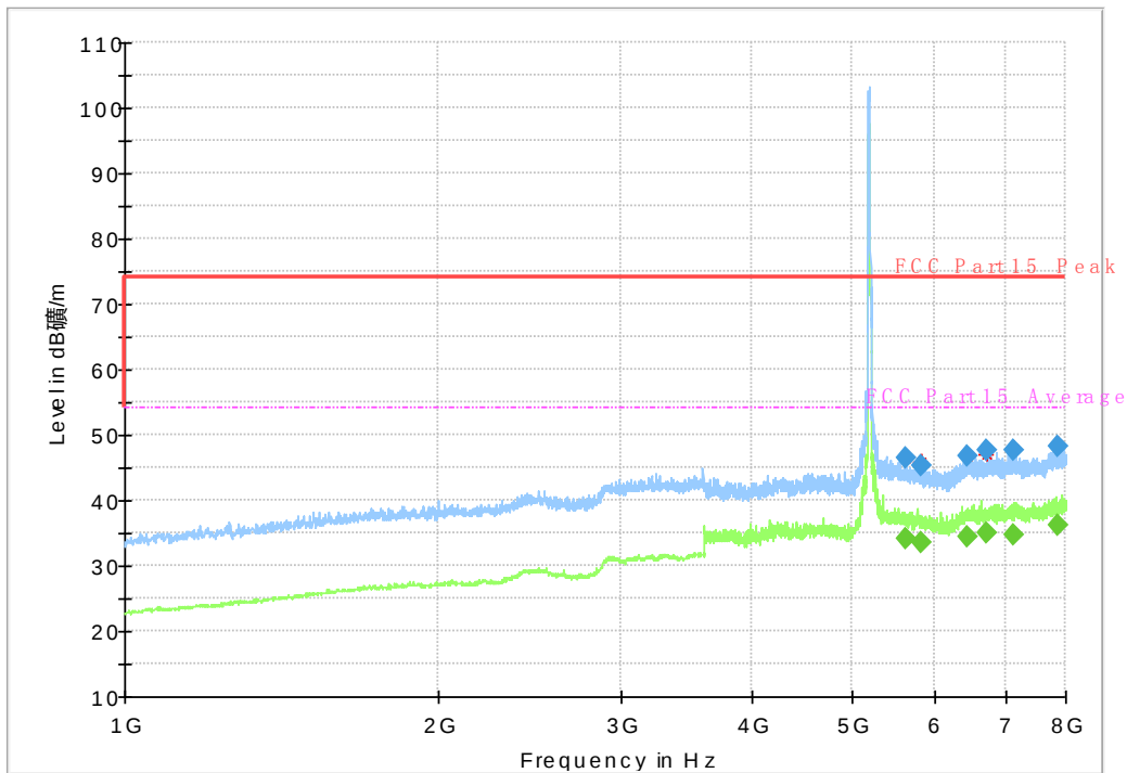
Fig. 45 Radiated Spurious Emission (802.11n-HT20, ch36, 1 GHz-8 GHz)
