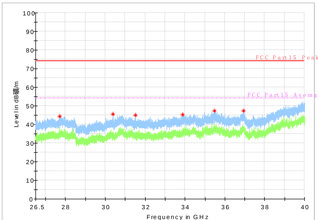
Fig. 53 Radiated Spurious Emission (802.11n-HT40, ch38, 26.5 GHz-40 GHz)
