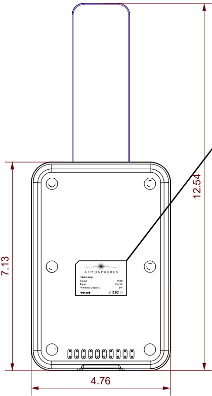
Bottom View
