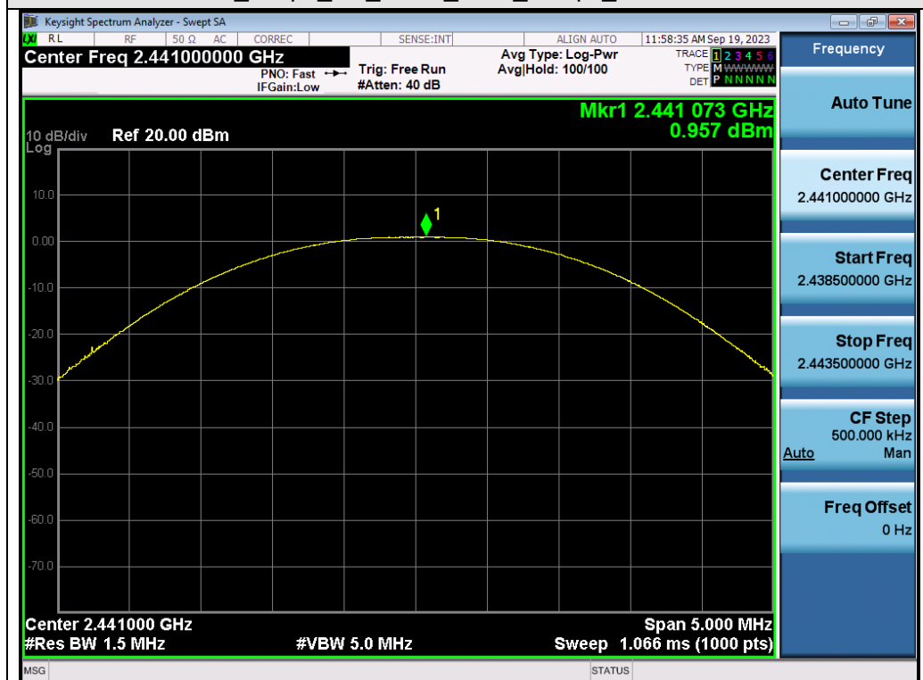
Test Graph BR ANT1 2441 1Mbps Peak Power
