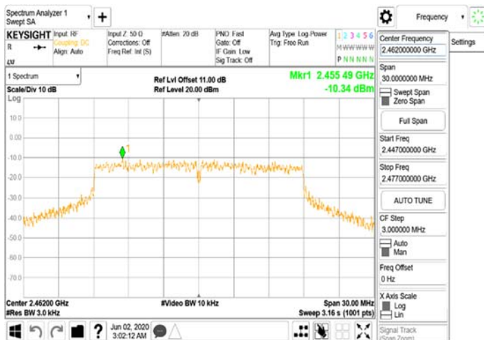
FCC_15_247_WLANPower Density_802.11n_20MHz_Chain0_2462MHz
