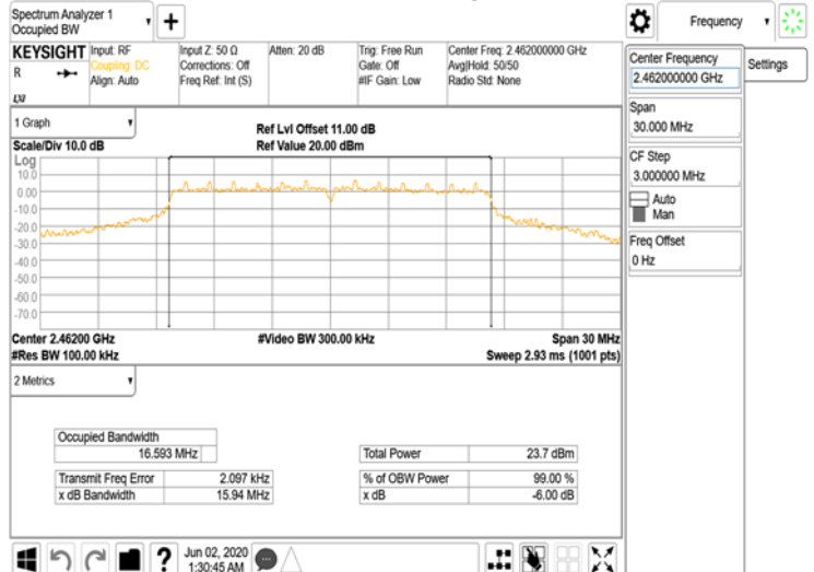
FCC_15_247_WLAN\OBW 6dB_802.11g_20MHz_Chain0_2462MHz
