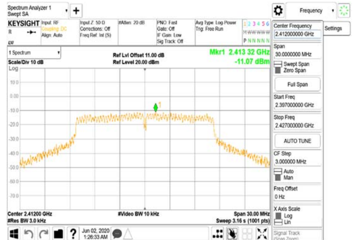
FCC_15_247_WLANPower Density_802.11g_20MHz_Chain0_2412MHz
