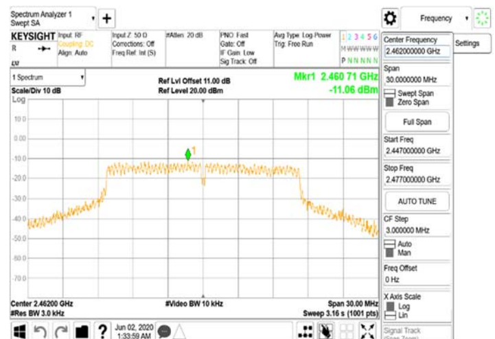
FCC_15_247_WLANPower Density_802.11g_20MHz_Chain0_2462MHz
