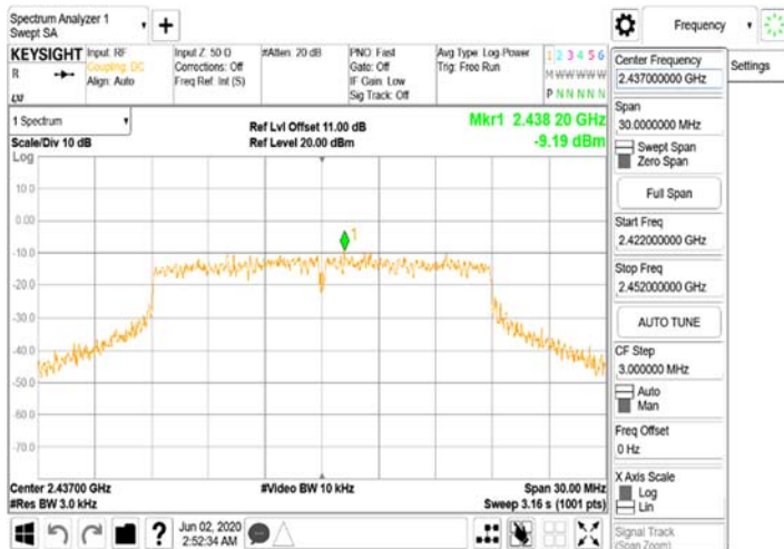
FCC_15_247_WLANPower Density_802.11n_20MHz_Chain0_2437MHz
