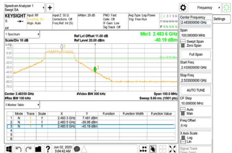
FCC_15_247_WLAN\Band Edge_802.11n_20MHz_Chain0_2462MHz
