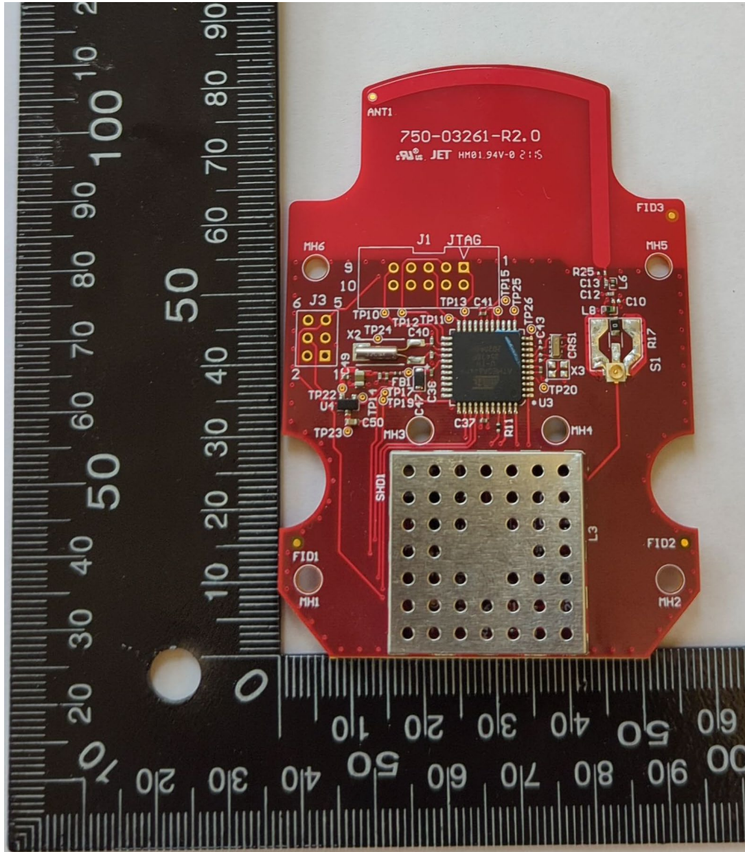
Trace Antenna
