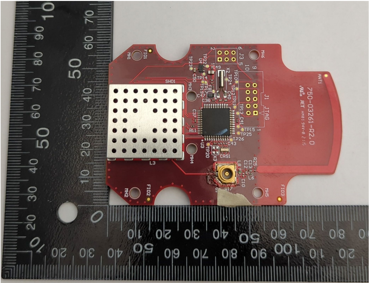
Board with Cable connection
