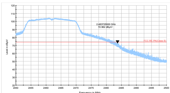
802.11g-Channel 11 Peak
