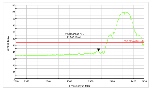
802.11b-Channel 1 Average
