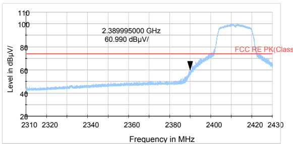
802.11g-Channel 1 Peak
