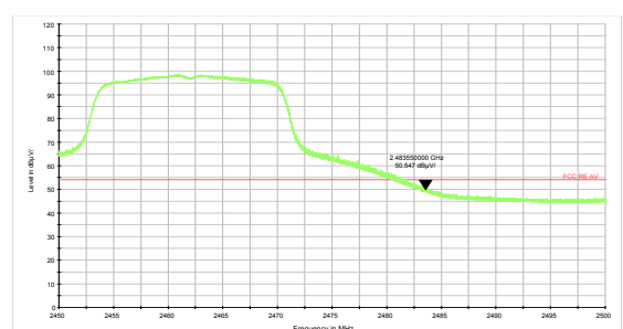
802.11g-Channel 11 Average
