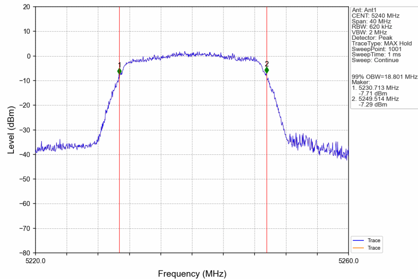
802.11ac(VHT20)_HCH_5240MHz_Ant1_NTNV
