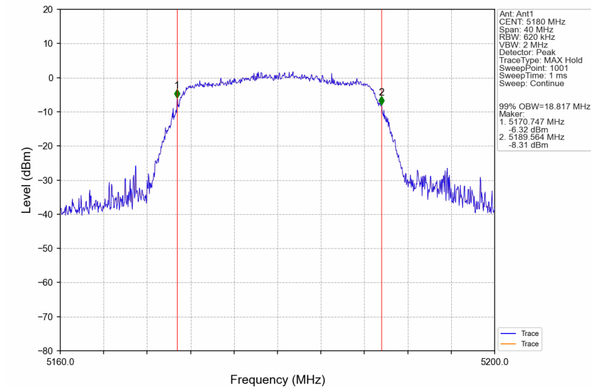
802.11ac(VHT20)_LCH_5180MHz_Ant1_NTNV
