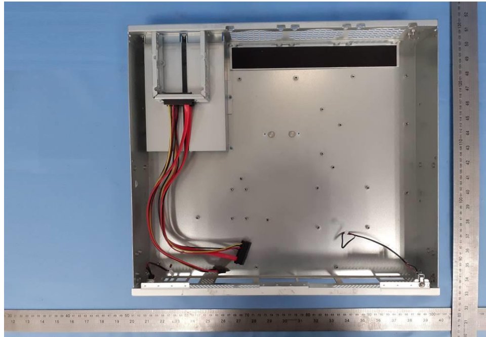
EUT Photo (39)
