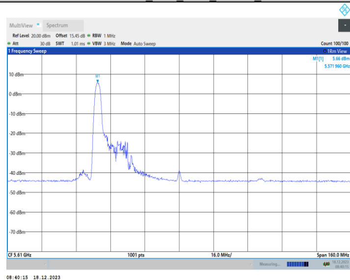
11AX80MIMO Ant2 5610 52Tone RU37
