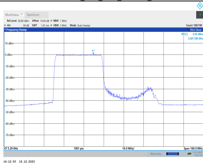
11AX80MIMO Ant2 5290 26Tone RU0
