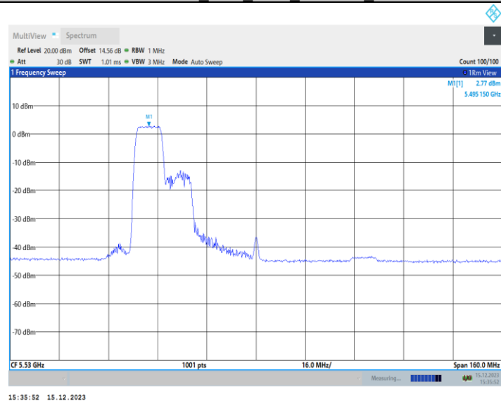
11AX80MIMO Ant1 5530 242Tone RU64
