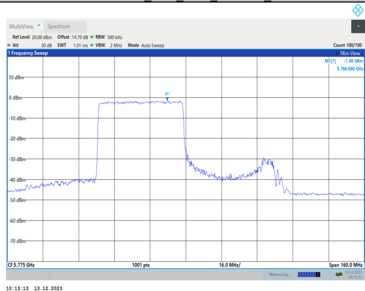
11AX80MIMO Ant2 5775 26Tone RU0
