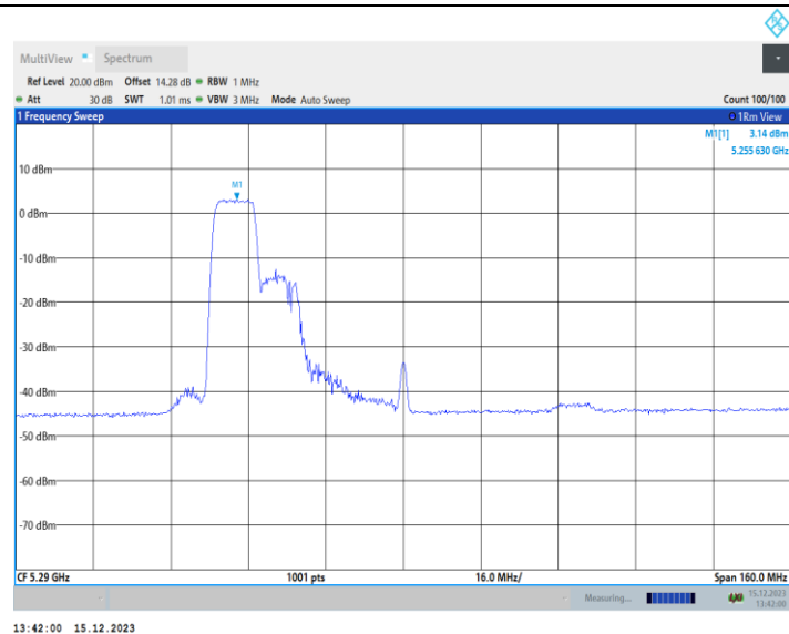
11AX80MIMO Ant1 5290 242Tone RU64
