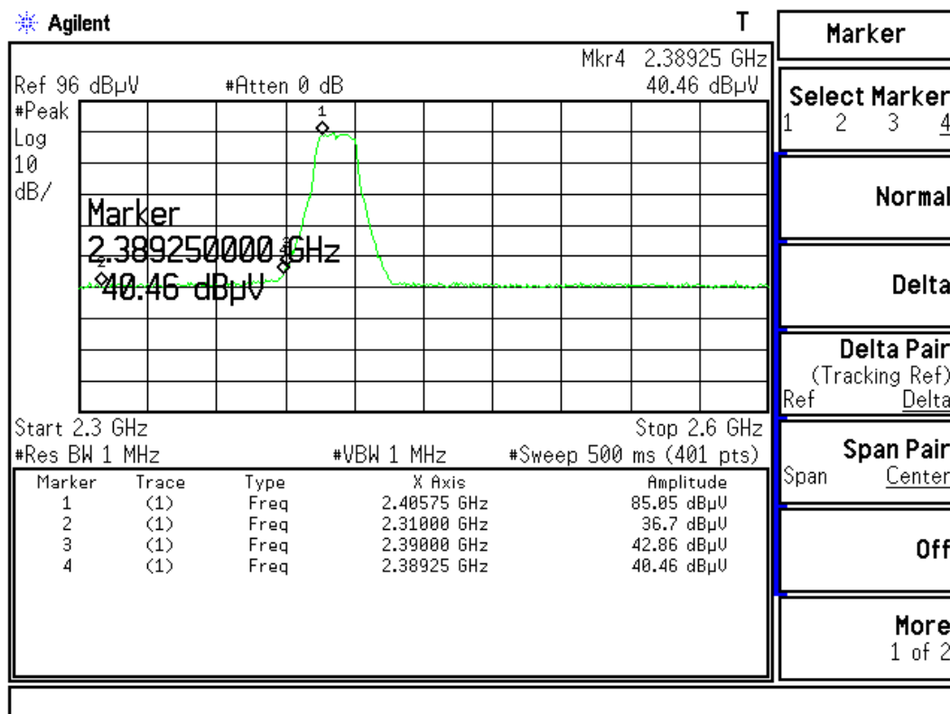
Figure Channel 1: (Horizontal)
