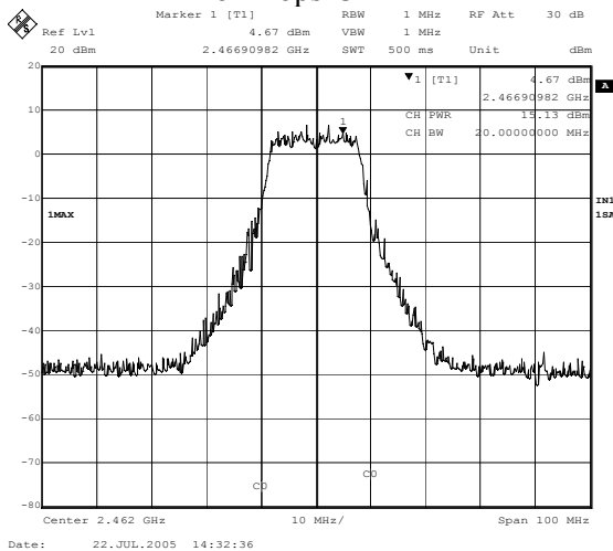
54Mbps-CH11
