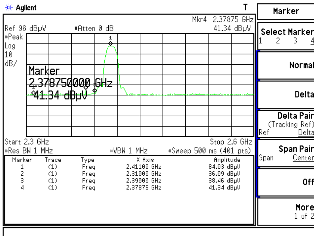
Figure Channel 1: (Vertical)
