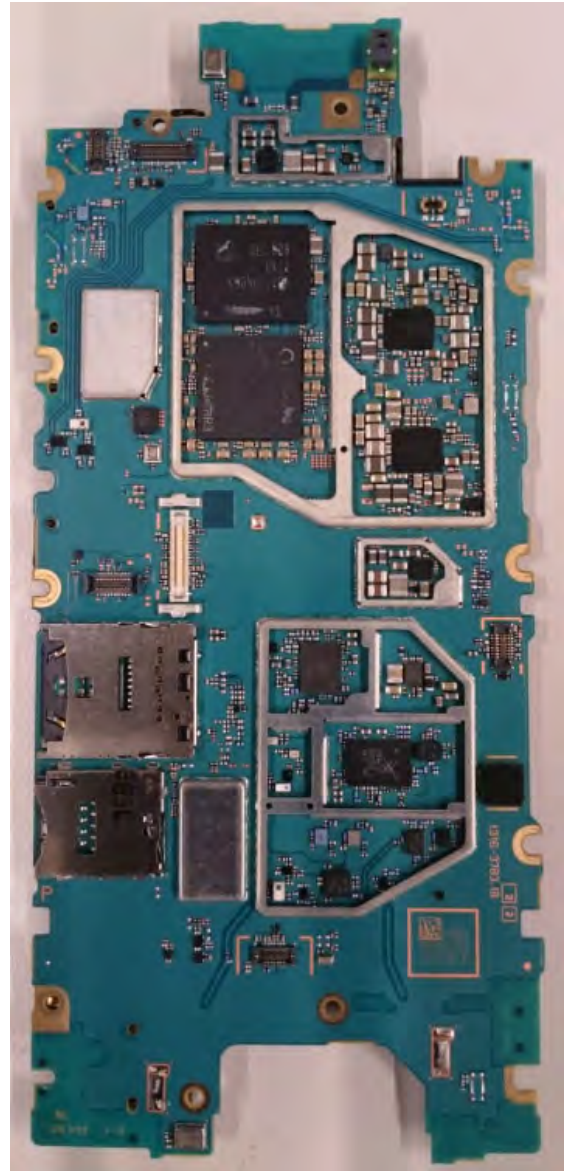
Internal PWB without Shield cases (Front-side)
