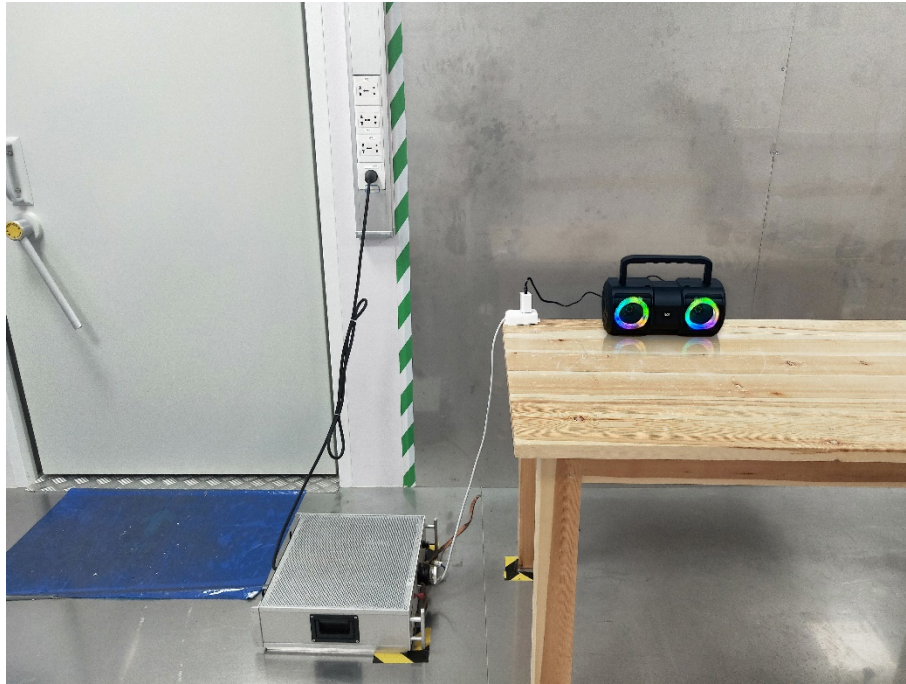
FCC: 2AJQ7BOOMX Photo of Conducted Emission Measurement
