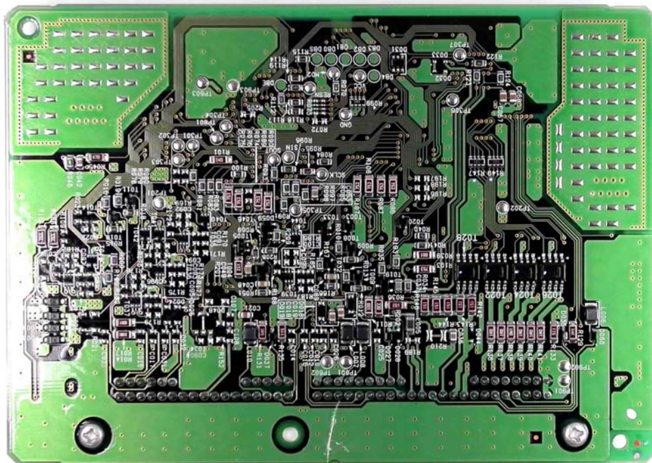
Computer Assy of TMLF-1 (PCB rear view)
