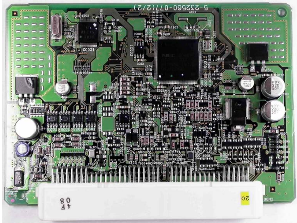
Computer Assy of TMLF-1 (PCB front view)
