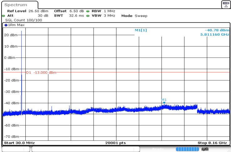
3MHz_Low_QPSK_15@0 -40.78 dBm
