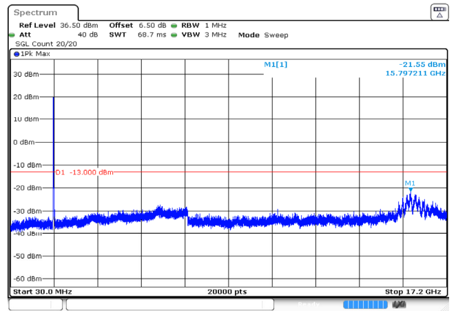
20MHz_Low_QPSK_1@0 -21.55dBm
