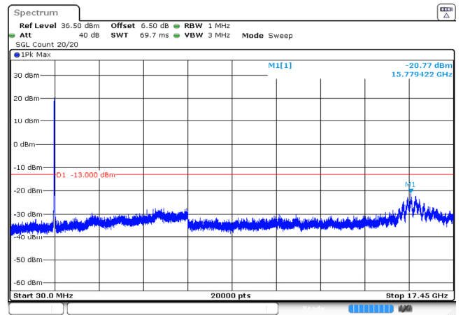
20MHz_High_QPSK_1@0 -20.77dBm
