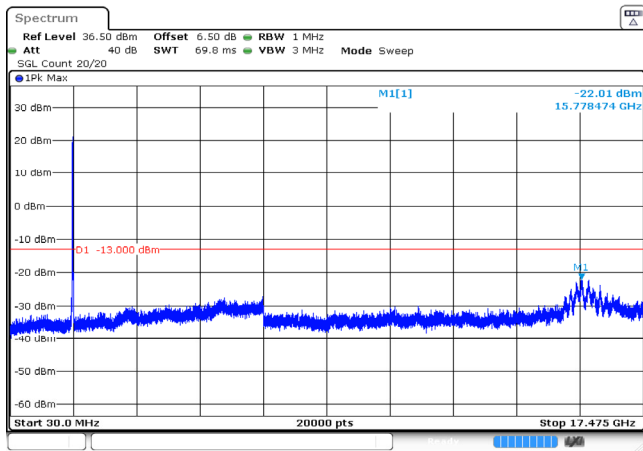
15MHz_High_QPSK_1@0 -22.01dBm
