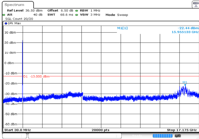
15MHz_Low_QPSK_1@0 -22.44dBm
