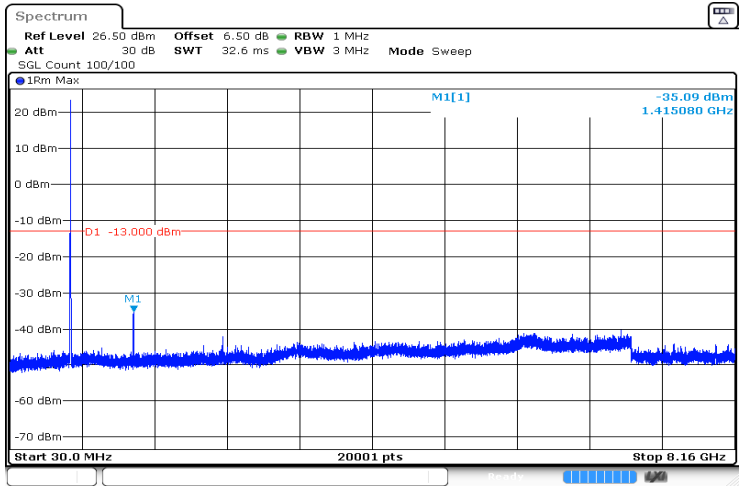
3MHz_Mid_QPSK_15@0 -35.09 dBm
