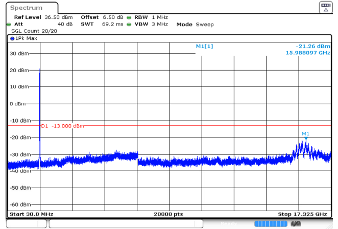
15MHz_Middle_QPSK_1@0 -21.26dBm
