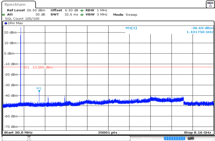
1.4MHz_High_QPSK_6@0 -36.69 dBm
