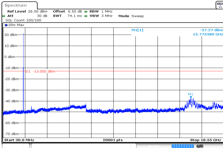
3MHz_Mid_QPSK_15@0 -37.27 dBm
