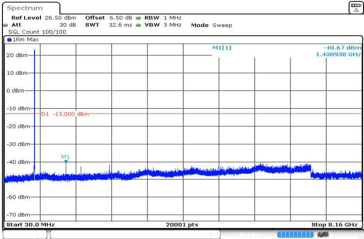
3MHz_High_QPSK_15@0 -40.67 dBm
