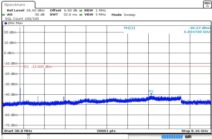
1.4MHz_Low_QPSK_6@0 -40.37 dBm
