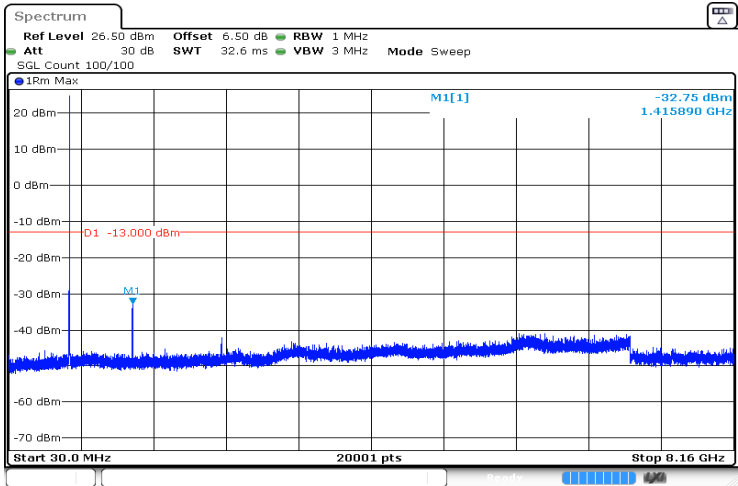
1.4MHz_Mid_QPSK_6@0 -32.75 dBm
