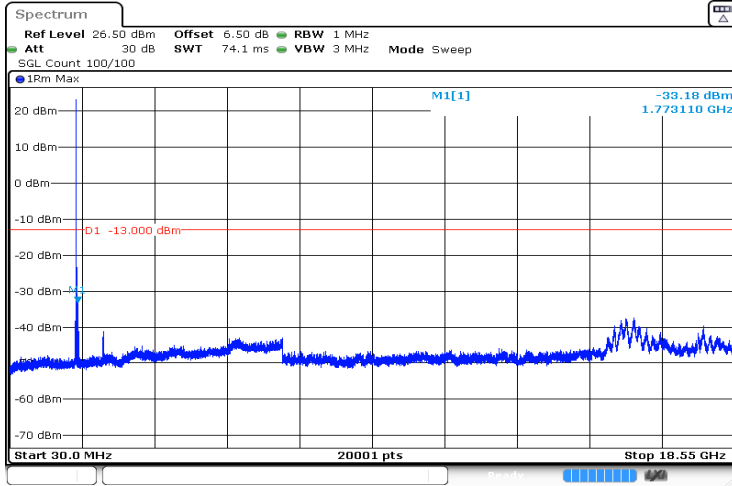
1.4MHz_Low_QPSK_6@0 -33.18 dBm
