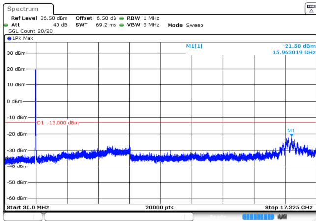
20MHz_Middle_QPSK_1@0 -21.58dBm
