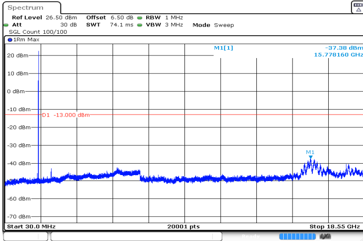
1.4MHz_High_QPSK_6@0 -37.38 dBm
