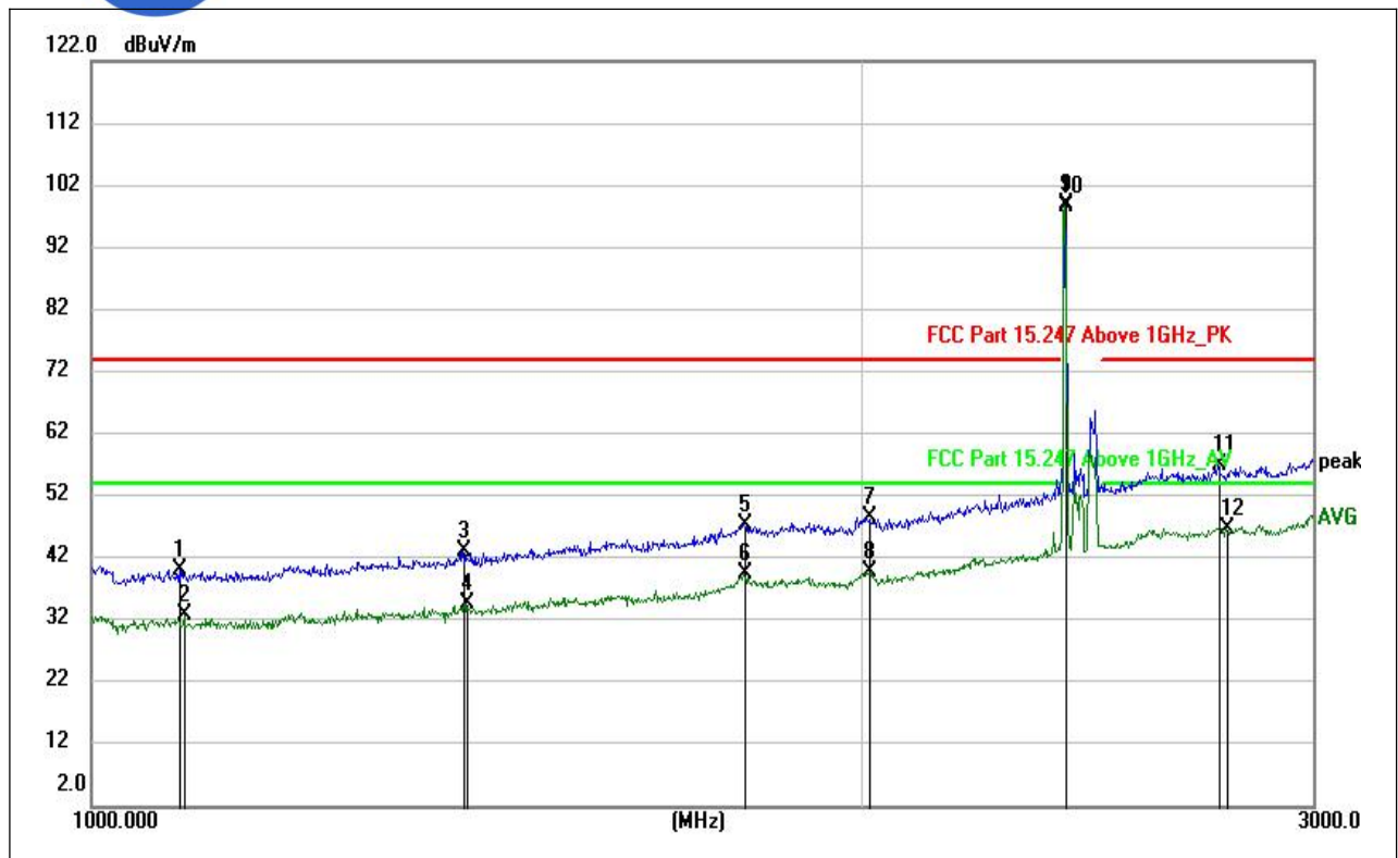
(LE 1M PHY _2402MHz, Antenna Horizontal, 1GHz to 3GHz)
