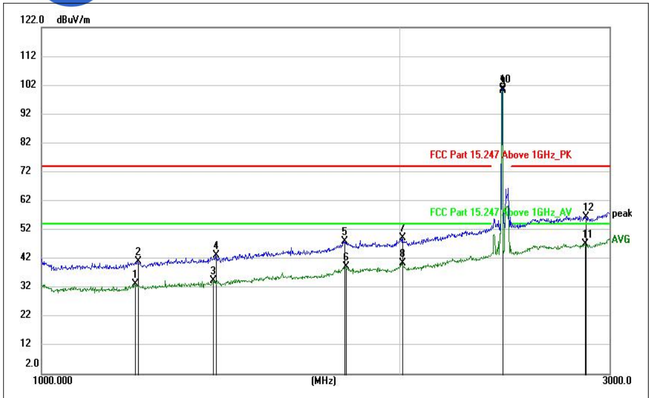
(LE 1M PHY _2442MHz, Antenna Vertical , 1GHz to 3GHz)
