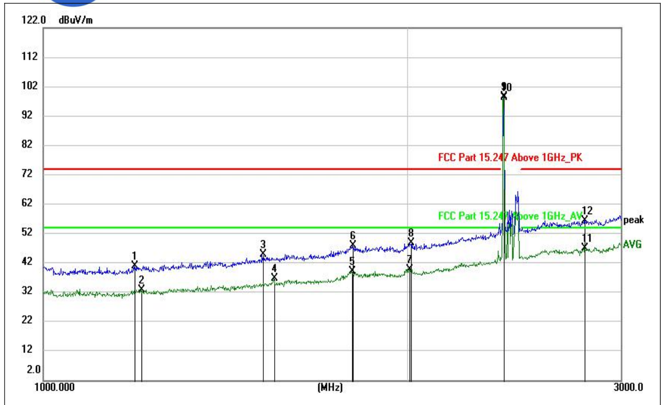
(LE 1M PHY _2402MHz, Antenna Vertical , 1GHz to 3GHz)
