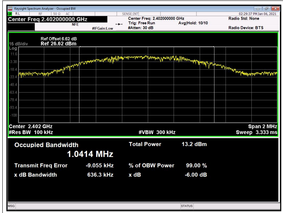
(Channel 0: 2402MHz)
