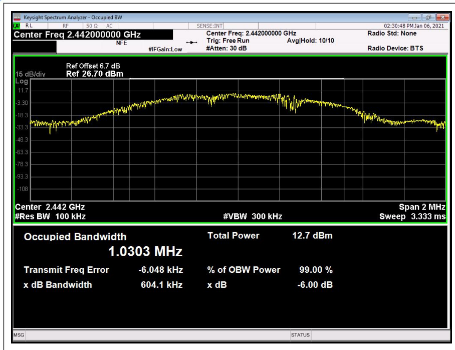
(Channel 20: 2442 MHz)
