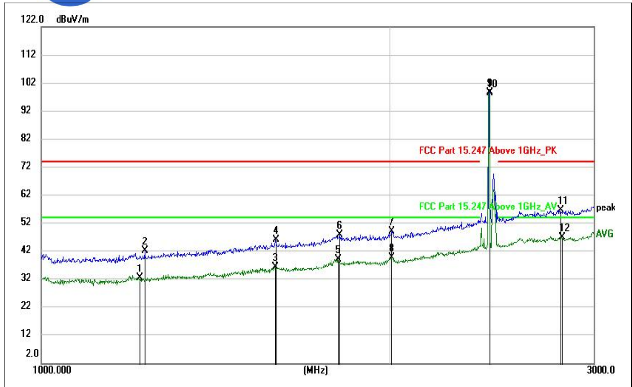
(LE 1M PHY _2442MHz, Antenna Horizontal, 1GHz to 3GHz)
