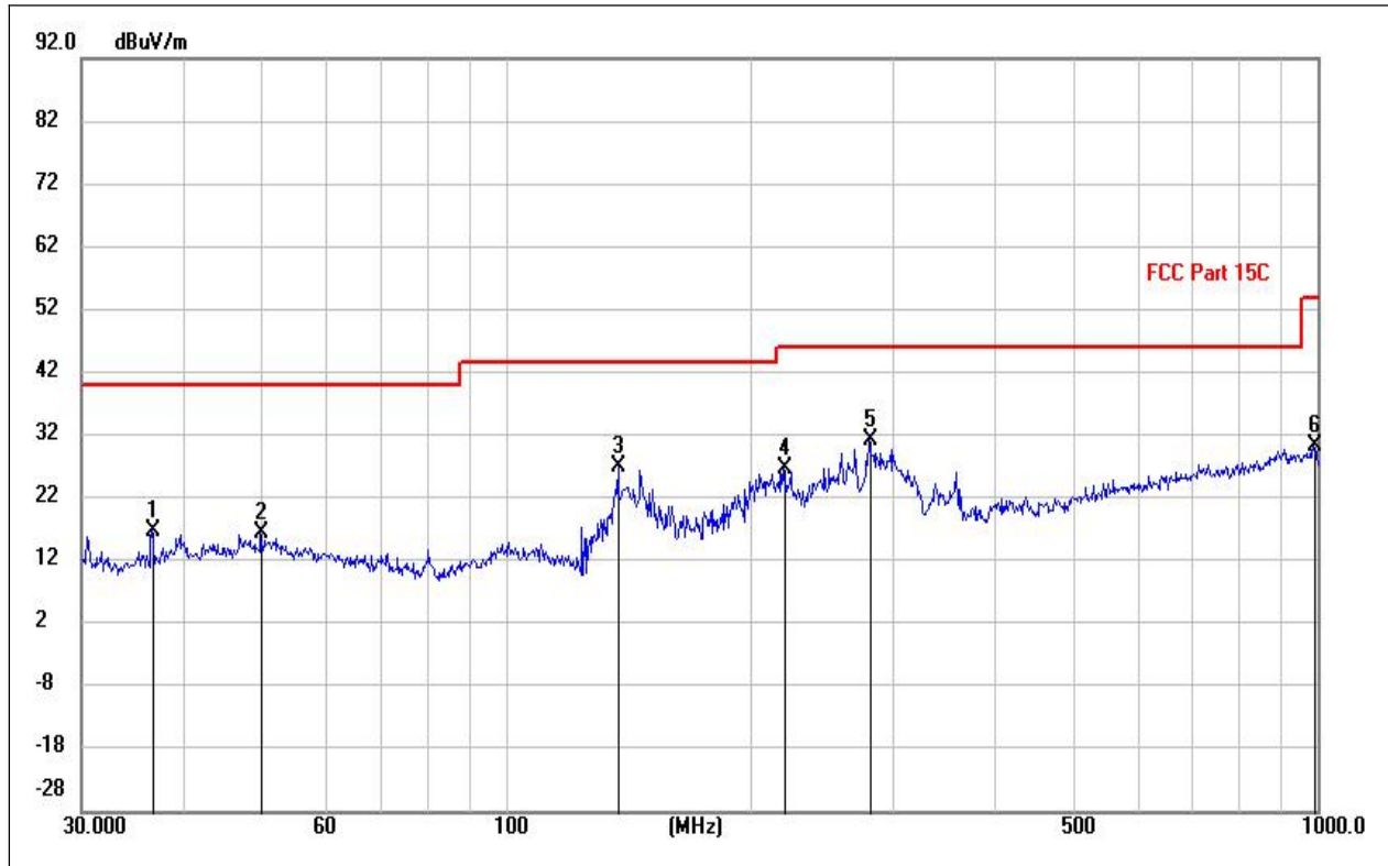
(LE 1M PHY_2402MHz, Antenna Horizontal, 30MHz to 1GHz)
