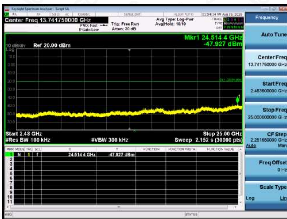
TEST PLOT OF OUT OF BAND EMISSIONS THE WORST CASE OF 802.11n20 FOR MODULATION IN HIGH CHANNEL
