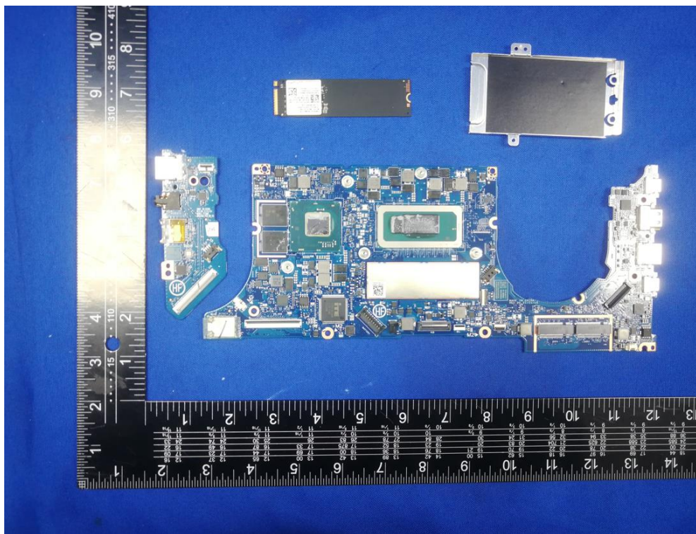
PWB view
