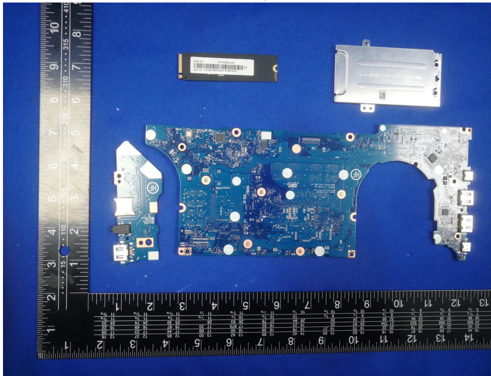
PWB view
