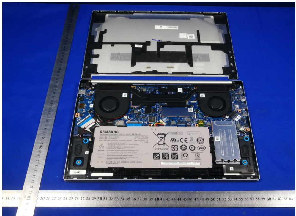
Internal view
