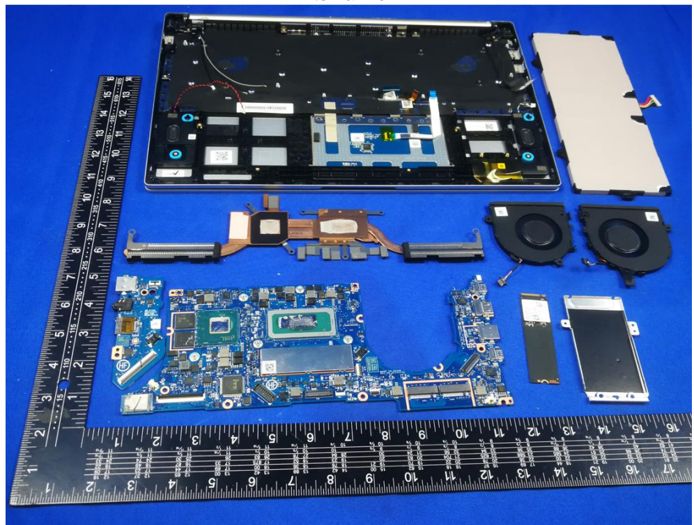
Internal view
