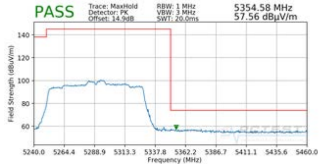
Plot 7-222. Radiated Upper Band Edge Plot SISO ANT2 (Peak – UNII Band 2A)
