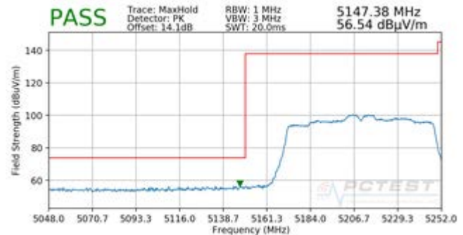
Plot 7-220. Radiated Lower Band Edge Plot SISO ANT2 (Peak – UNII Band 1)
