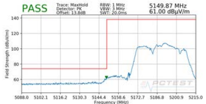
Plot 7-238. Radiated Lower Band Edge Plot MIMO (Peak – UNII Band 1)
