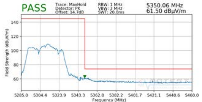
Plot 7-240. Radiated Upper Band Edge Plot MIMO (Peak – UNII Band 2A)
