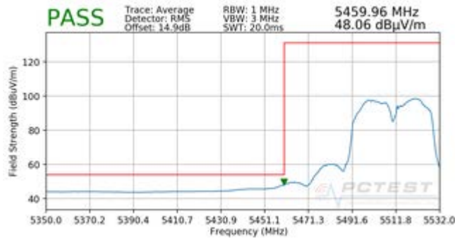
Plot 7-241. Radiated Lower Band Edge Plot MIMO (Average – UNII Band 2C)
