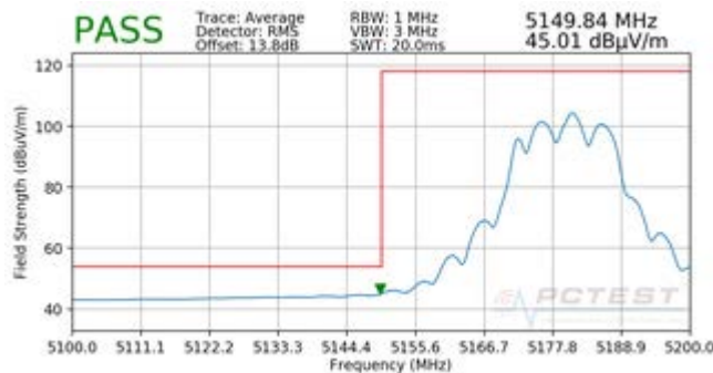
Plot 7-228. Radiated Lower Band Edge Plot CDD (Average – UNII Band 1)
