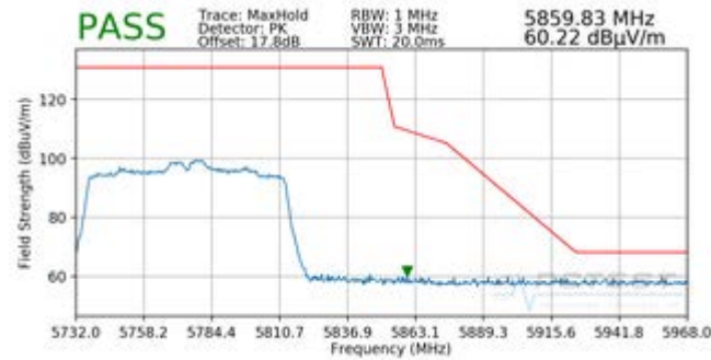
Plot 7-198. Radiated Upper Band Edge Plot SISO ANT1 (Peak – UNII Band 3)
