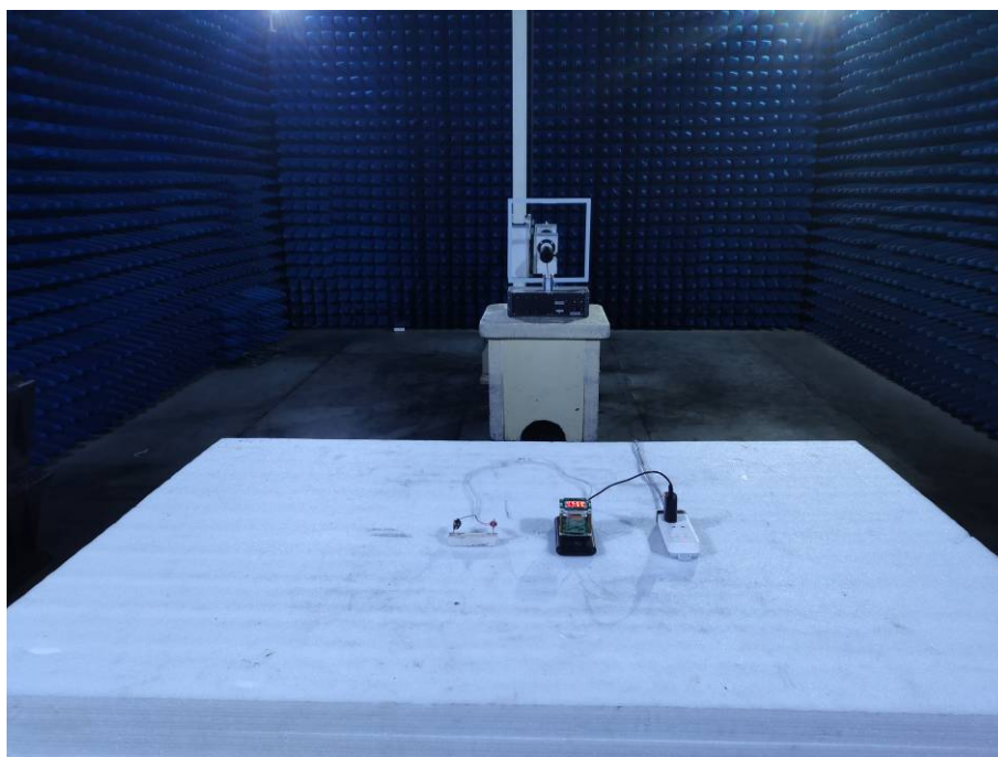
Photo of Radiated Emission Measurement (9k-30MHz)
