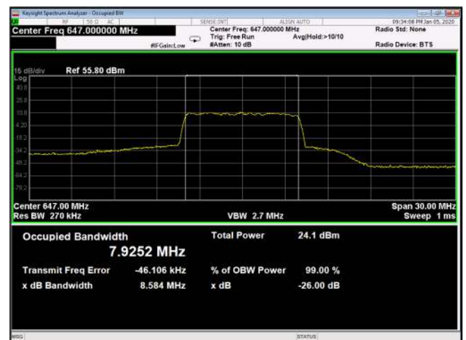
Figure 538: 64QAM 10MHz B.W; 647.0 MHz, 60kHz Output
