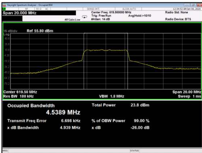
Figure 557: 256QAM 5MHz B.W; 619.5MHz, 15kHz Output
