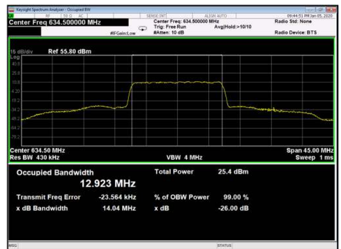
Figure 544: 64QAM 15MHz B.W; 634.5MHz, 60kHz Output
