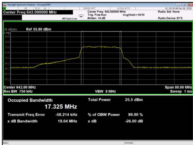
Figure 589: 256QAM 20MHz B.W; 642.0MHz, 60kHz Output
