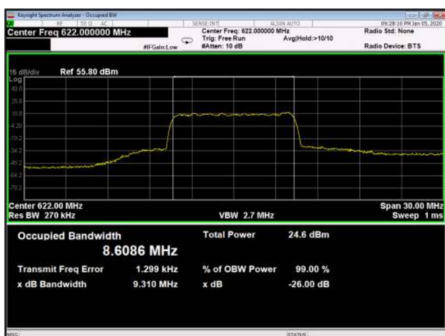
Figure 531: 64QAM 10MHz B.W; 622.0MHz, 60kHz Output
