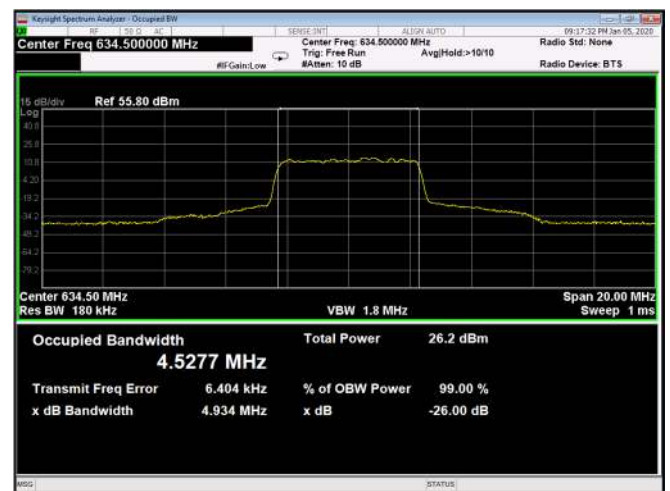
Figure 526: 64QAM 5MHz B.W; 634.5MHz, 15kHz Output
