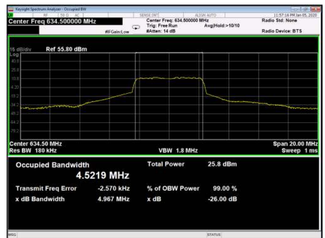
Figure 592: QPSK 5MHz B.W; 634.5MHz, 15kHz Output
