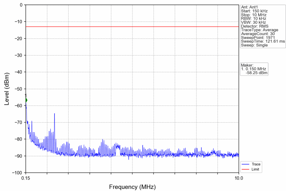
Band13_10MHz_QPSK_MCH_782MHz_RB_1_0_NTNV
