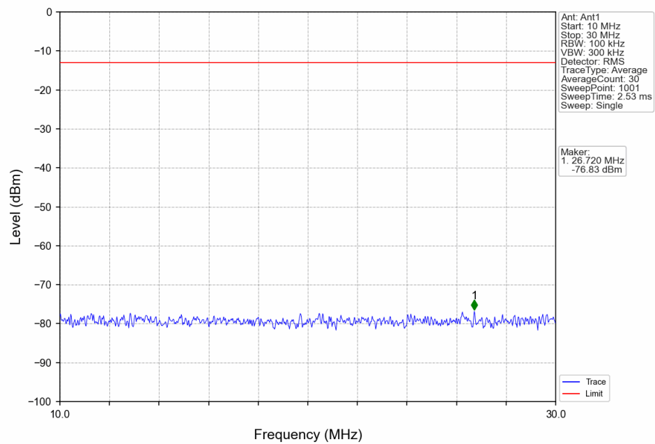
Band13_10MHz_QPSK_MCH_782MHz_RB_1_0_NTNV
