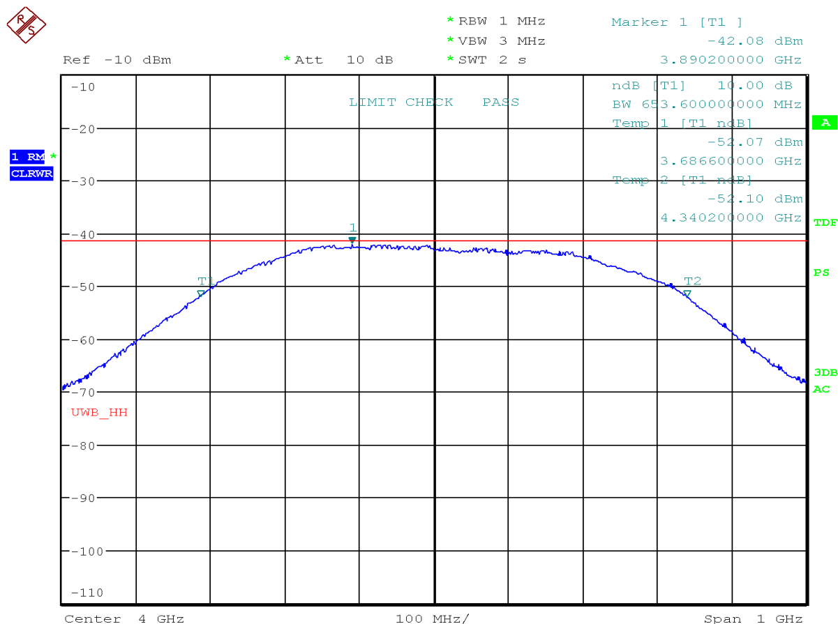
Horizontal Bandwidth Plot
