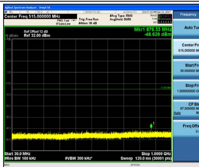
Band4_1.4MHz_QPSK_20175_1RB#0
