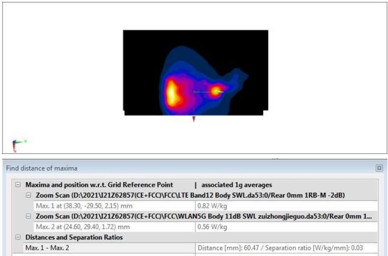
Picture 15.3-1 Distance evaluation for LTE B12 and WiFi 5G
