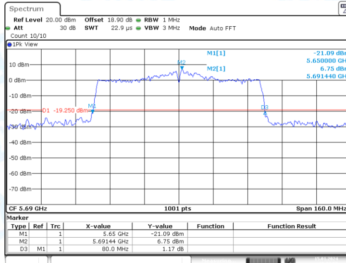
11AC80-CDD_Ant2_5690
