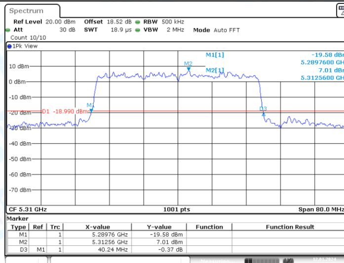
11AX40-CDD_Ant2_5310
