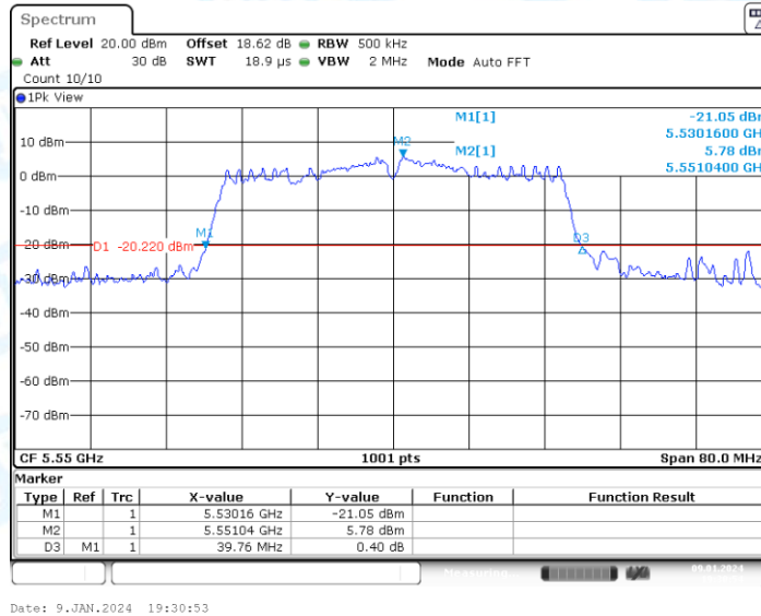
11AC40-CDD_Ant2_5550
