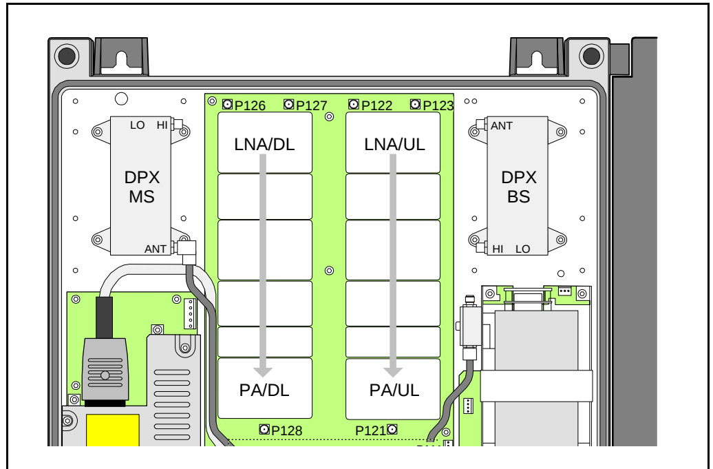
Figure 5-4. LNA, Low Noise Amplifiers
