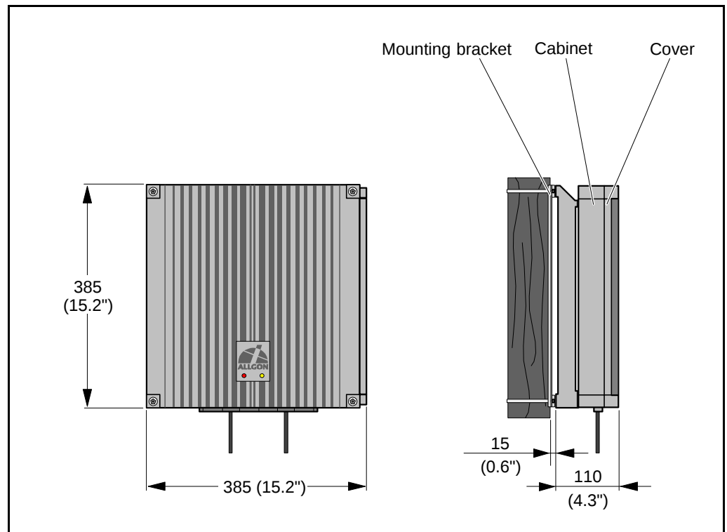
Figure 3-1. Repeater dimensions
