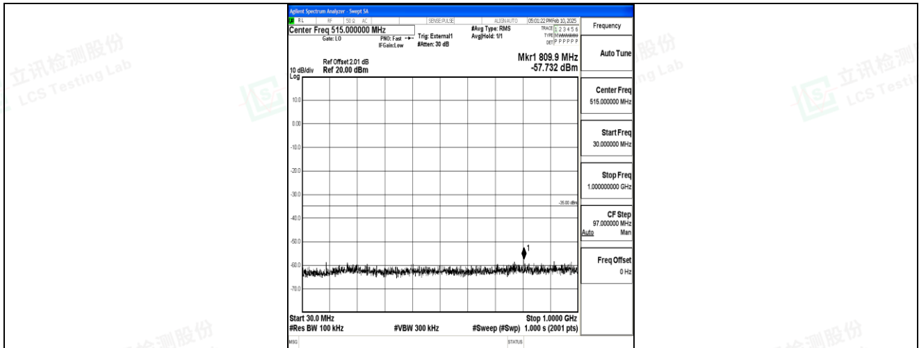
Band41_15MHz_QPSK_41515_1RB#0_30~1000_30~1000
