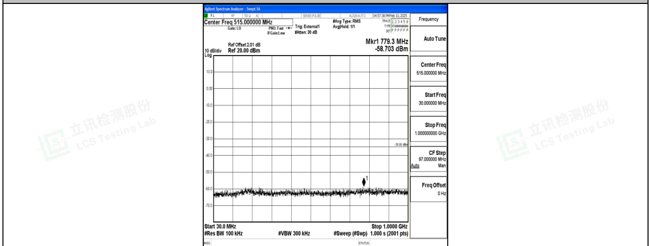
Band41_15MHz_QPSK_40620_1RB#0_30~1000_30~1000
