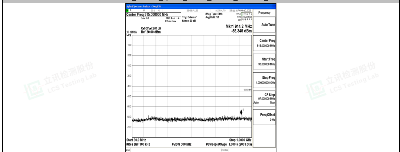
Band41_20MHz_QPSK_40620_1RB#0_30~1000_30~1000
