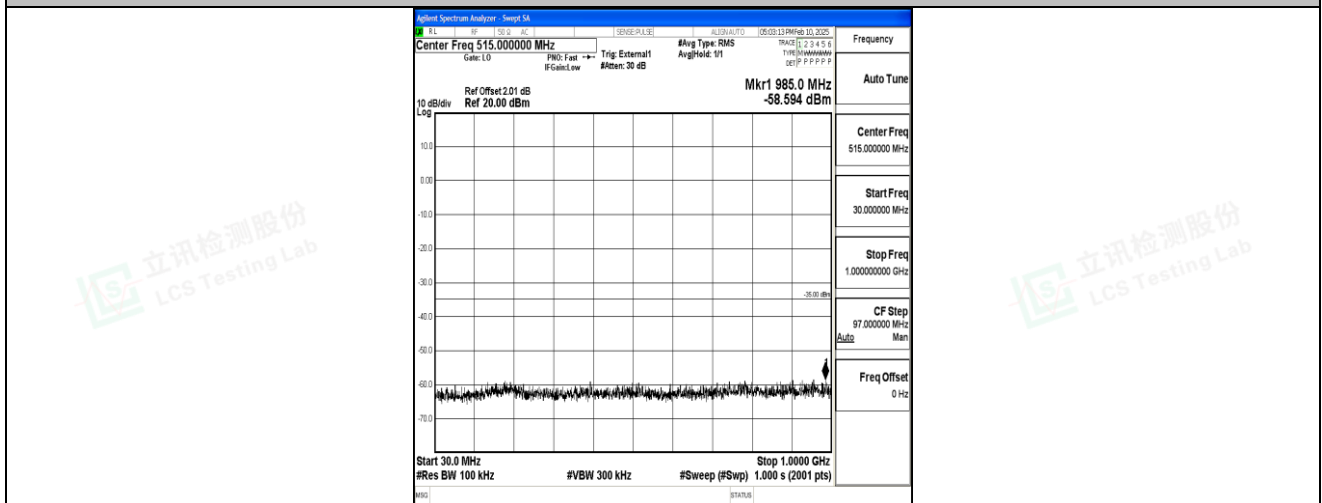
Band41_15MHz_16QAM_41515_1RB#0_30~1000_30~1000
