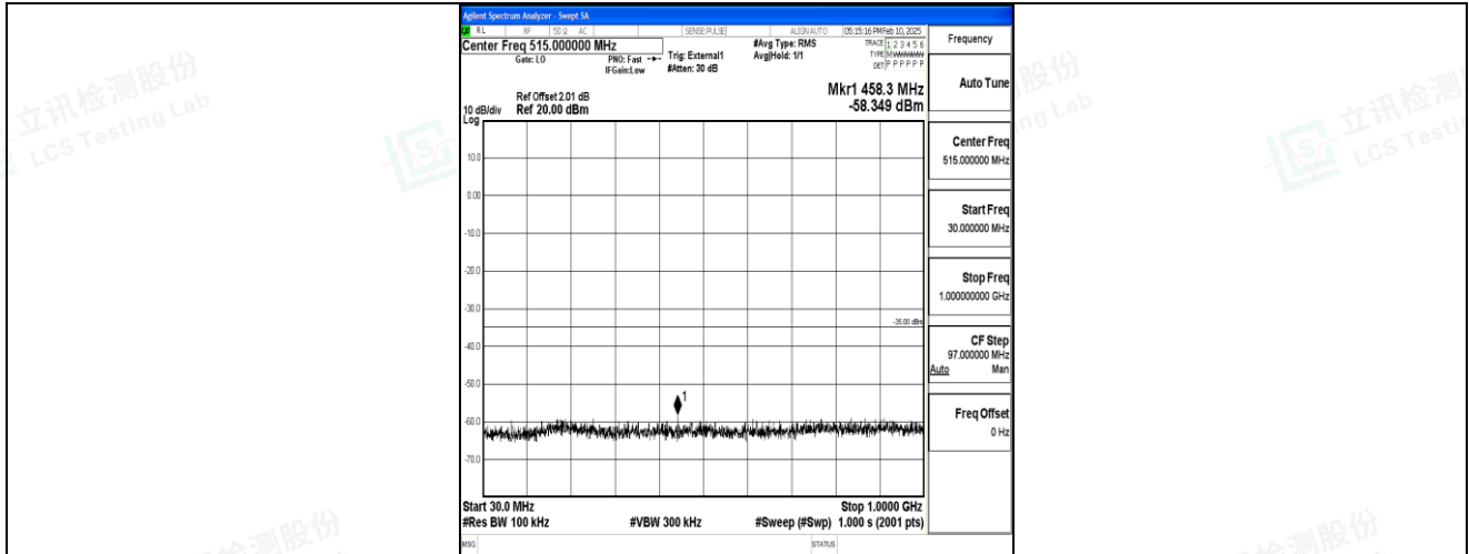
Band41_20MHz_QPSK_41490_1RB#0_30~1000_30~1000
