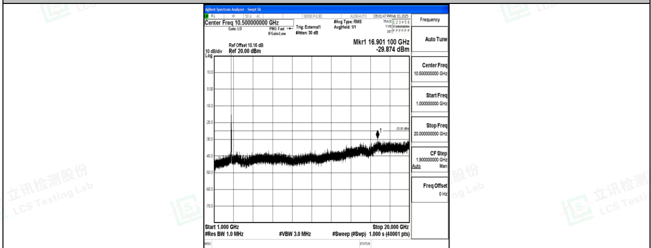
Band41_15MHz_QPSK_41515_1RB#0_1000~20000_1000~20000
