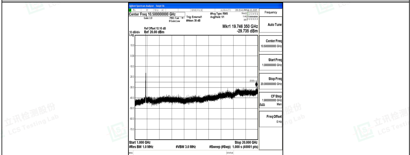
Band41_20MHz_QPSK_41490_1RB#0_1000~20000_1000~20000
