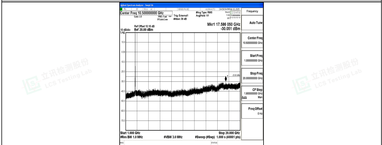
Band41_15MHz_16QAM_40620_1RB#0_1000~20000_1000~20000
