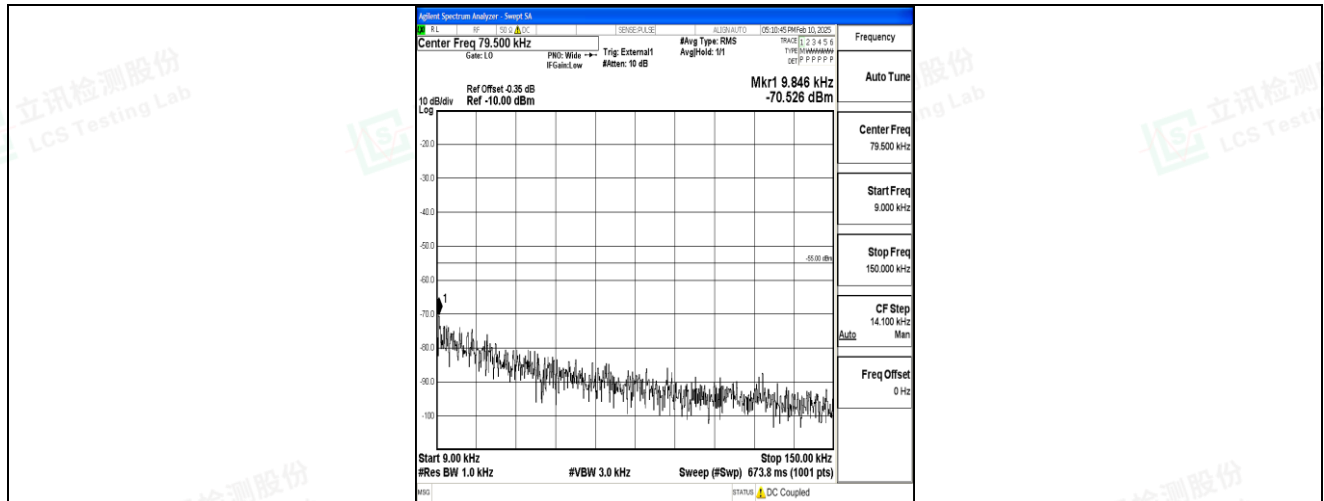
Band41_20MHz_QPSK_40620_1RB#0_0.009~0.15_0.009~0.15
