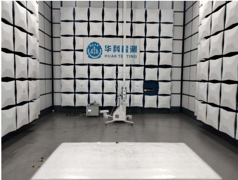
Model: YS-TWS095 Radiated Emissions
