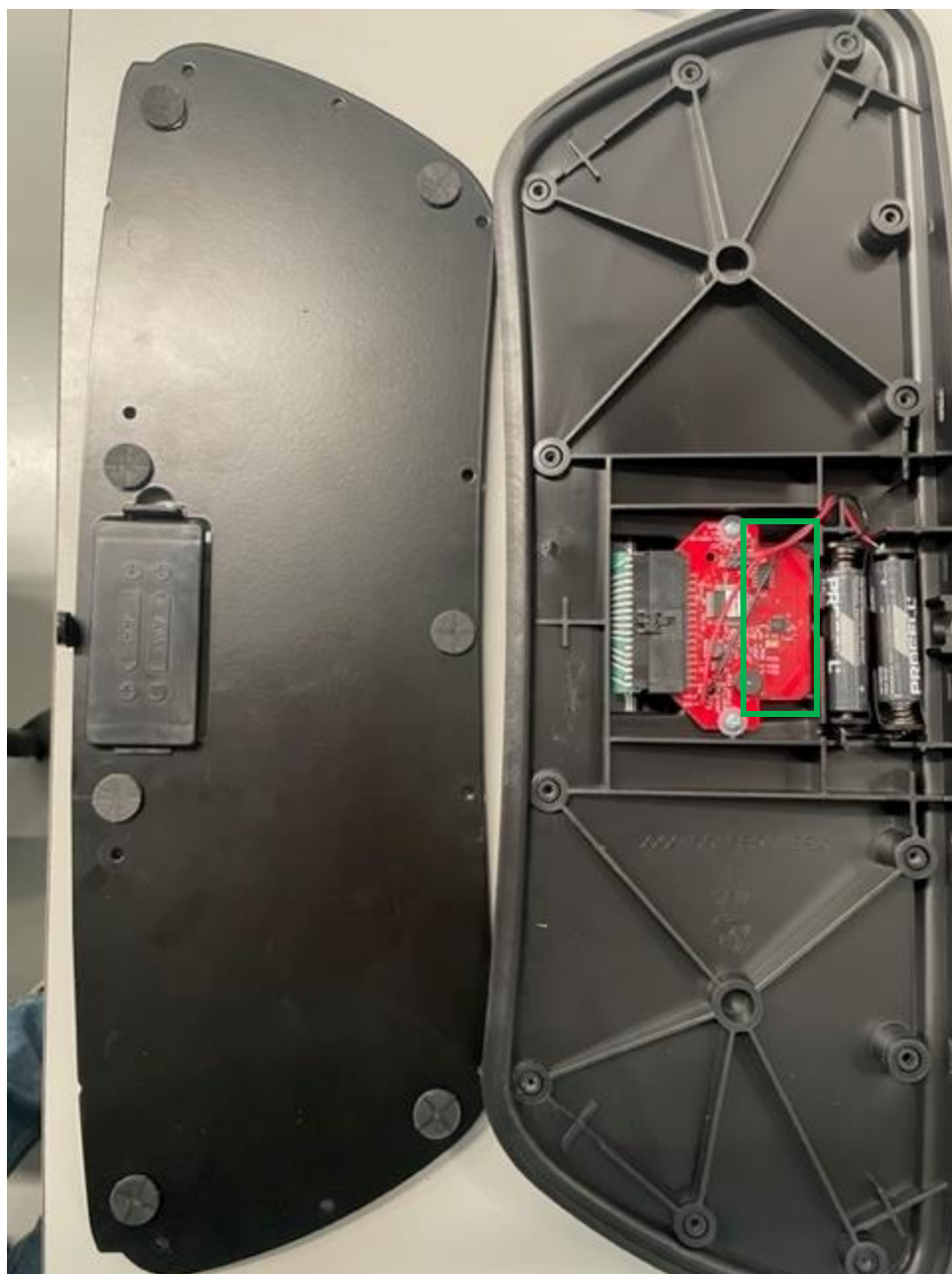
Figure 1: Inside of the Wireless Remote Foot Control Antenna location is denoted by the green square.
