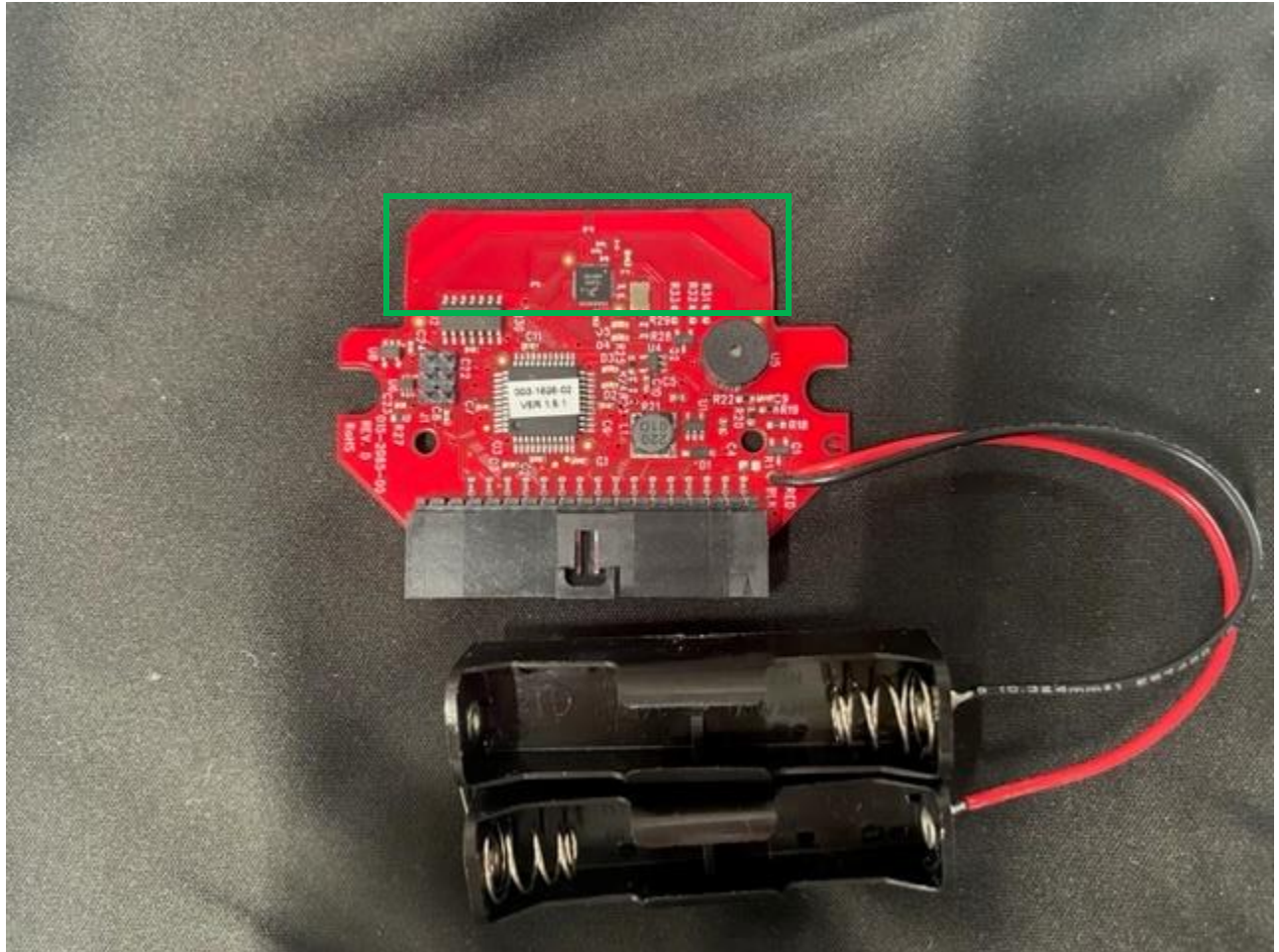
Figure 2: Top Side of the Wireless Remote Foot Control PCB Antenna location is denoted by the green square.
