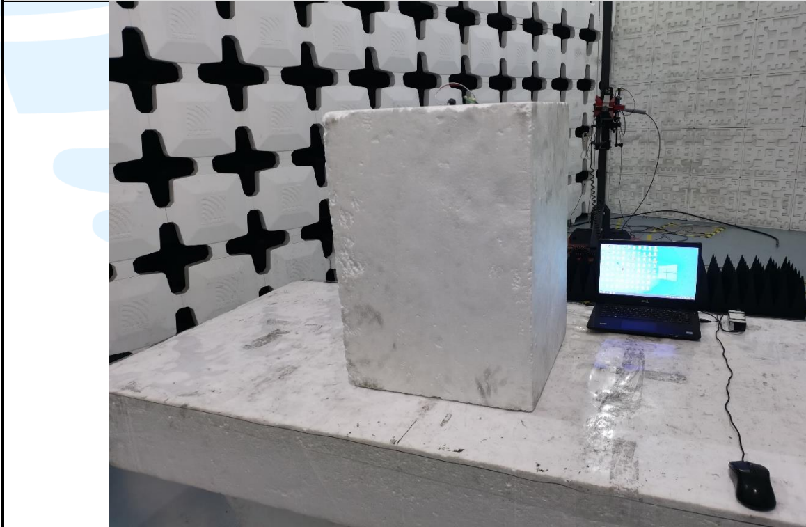
Radiated emission Test Setup (Above 1 GHz) _Right earbuds
