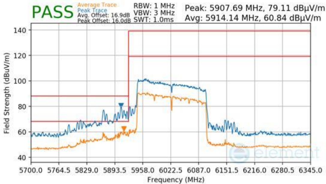
Plot 7-2082 Antenna 1b Radiated Lower Band Edge (Peak/Average – UNII Band 5 – RU996x2)
