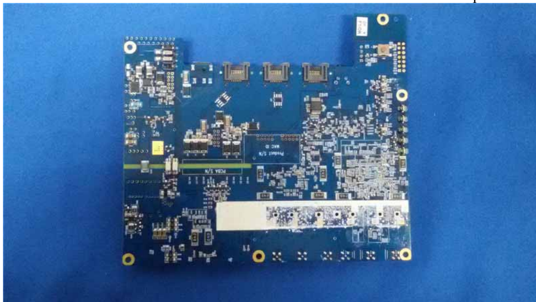
Figure 11 Component Side of the PCB
