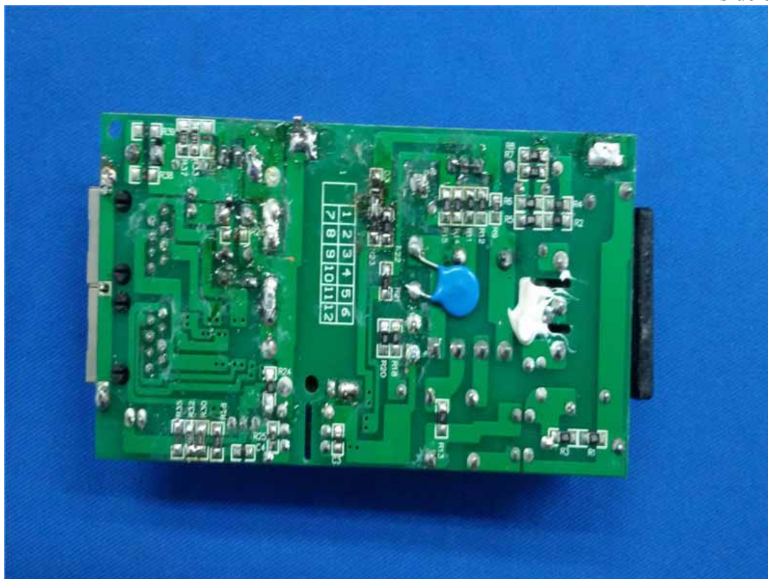
Figure 24 Inside of the Adapter
