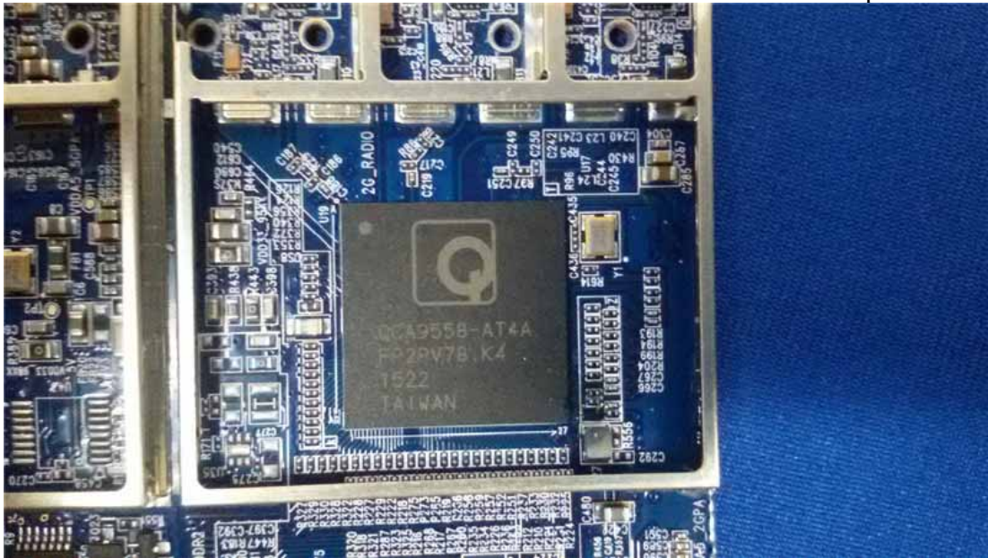
Figure 16 Component Side of the PCB
