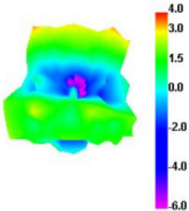
5300MHz 3D Antenna pattern
