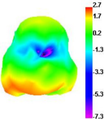
3D Antenna pattern
