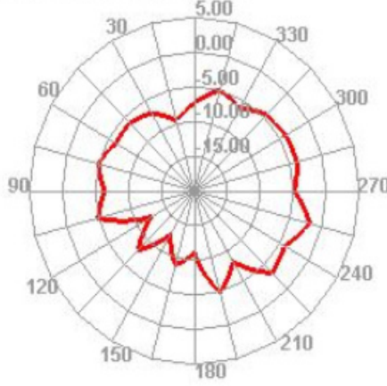
2D Antenna pattern (X->Y;X->Z;Y->Z)
