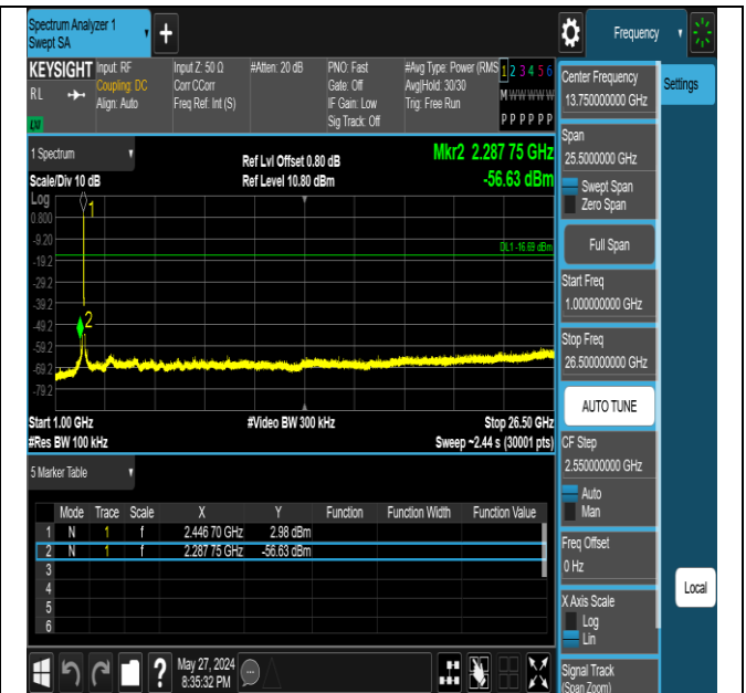
11N40SISO-Ant1-2452-1000~26500-PASS
