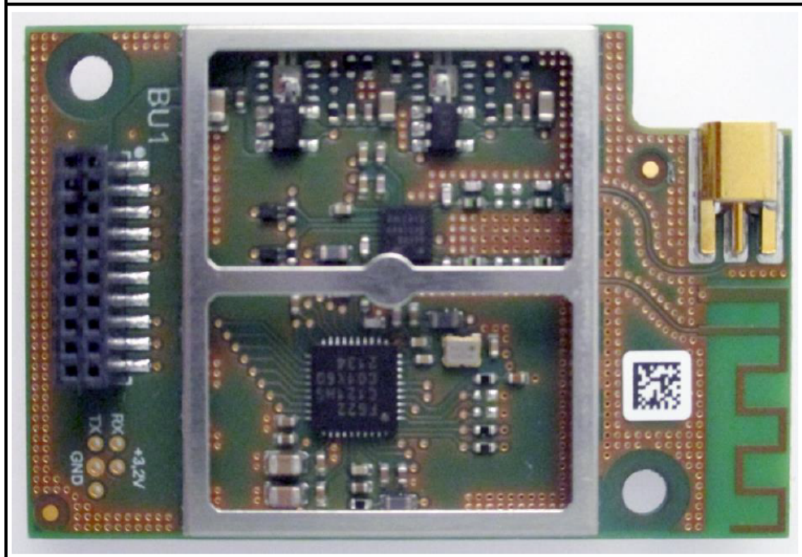
TC242C01_EUT5.2 - radiated sample without shielding
