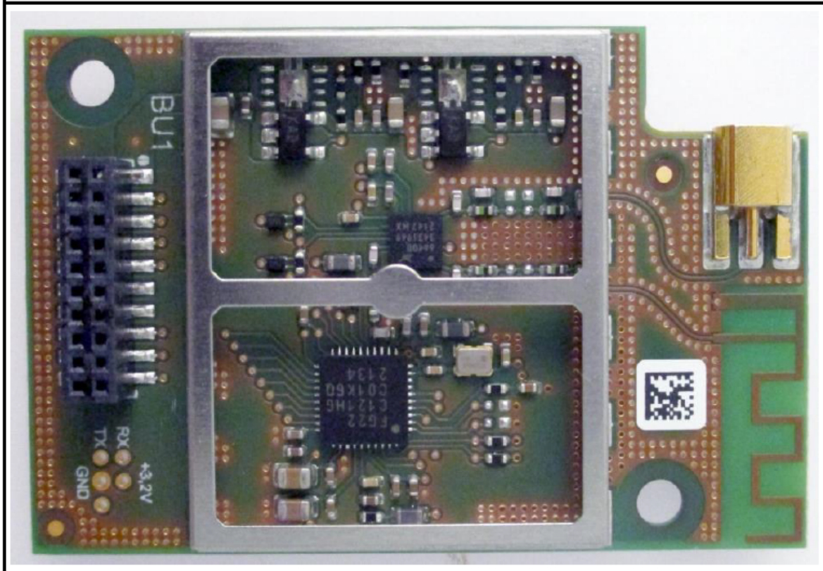
TC242C01_EUT7.2 – conducted sample without shielding
