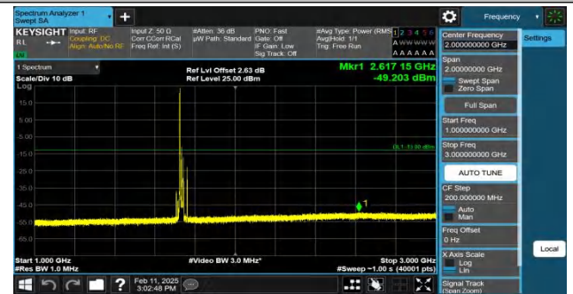
Band4-20MHz-QPSK-20175-1RB#0-1000~3000-PASS
