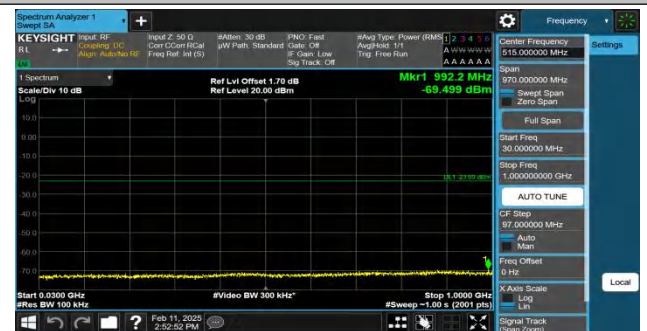
Band4-15MHz-QPSK-20025-1RB#74-30~1000-PASS
