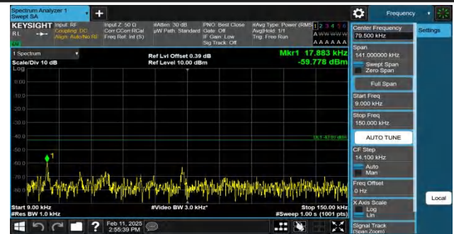
Band4-15MHz-QPSK-20325-1RB#74-0.009~0.15-PASS
