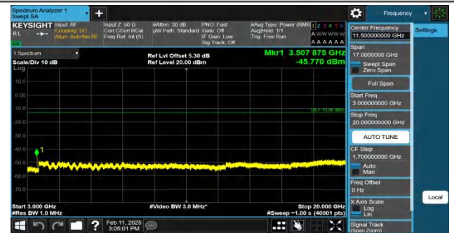
Band4-20MHz-QPSK-20300-1RB#99-3000~20000-PASS
