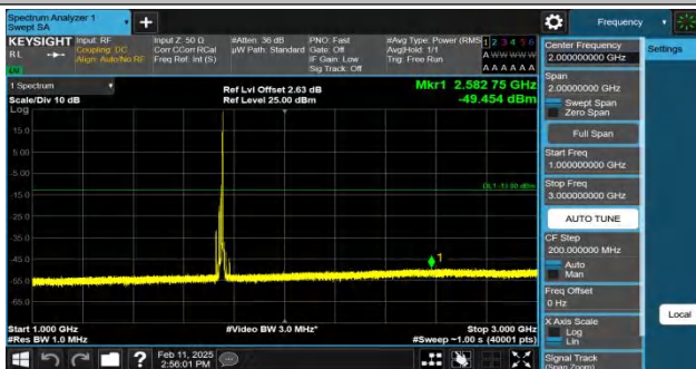
Band4-15MHz-QPSK-20325-1RB#74-1000~3000-PASS
