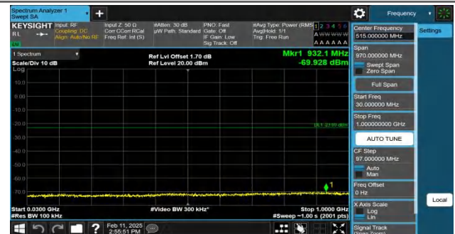
Band4-15MHz-QPSK-20325-1RB#74-30~1000-PASS
