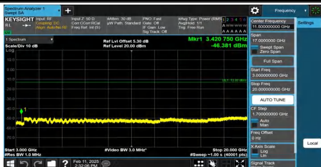
Band4-5MHz-QPSK-19975-1RB#0-3000~20000-PASS
