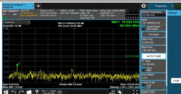
Band4-5MHz-QPSK-20175-1RB#0-0.009~0.15-PASS
