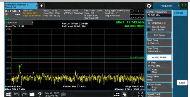
Band4-15MHz-QPSK-20025-1RB#74-0.009~0.15-PASS
