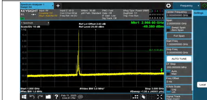
Band4-20MHz-QPSK-20300-1RB#99-1000~3000-PASS
