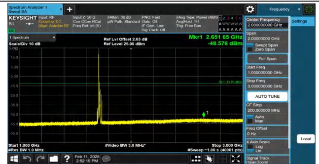
Band4-15MHz-QPSK-20025-1RB#0-1000~3000-PASS
