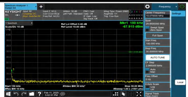
Band4-20MHz-QPSK-20175-1RB#0-0.15~30-PASS
