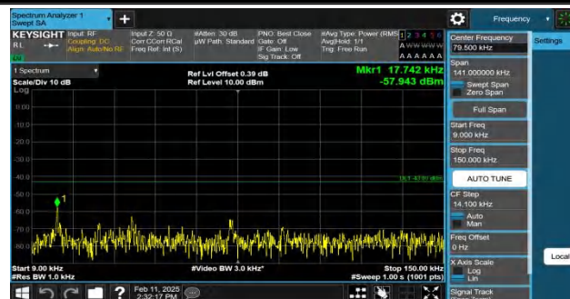
Band4-5MHz-QPSK-19975-1RB#24-0.009~0.15-PASS
