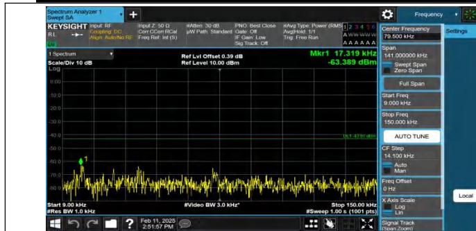
Band4-15MHz-QPSK-20025-1RB#0-0.009~0.15-PASS
