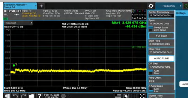
Band4-5MHz-QPSK-19975-1RB#24-3000~20000-PASS
