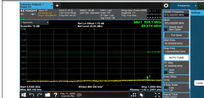
Band4-20MHz-QPSK-20175-1RB#0-30~1000-PASS
