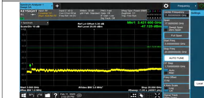
Band4-15MHz-QPSK-20025-1RB#0-3000~20000-PASS
