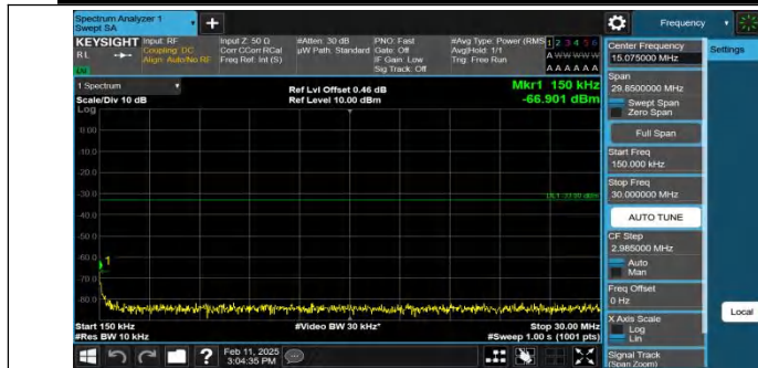
Band4-20MHz-QPSK-20300-1RB#99-0.15~30-PASS
