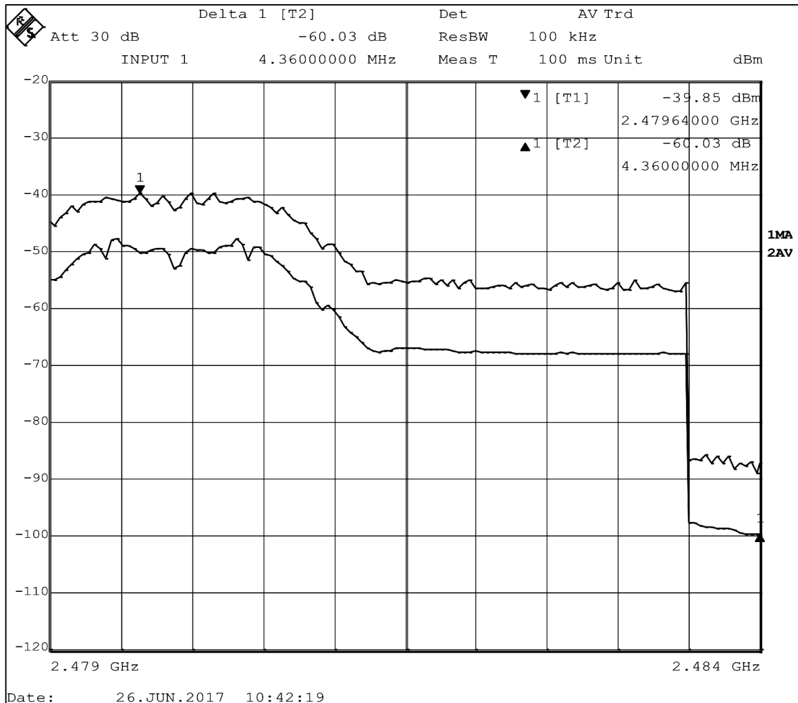
Figure 14 - Band-edge Measurement, High Channel, Restricted and Unrestricted Frequency
