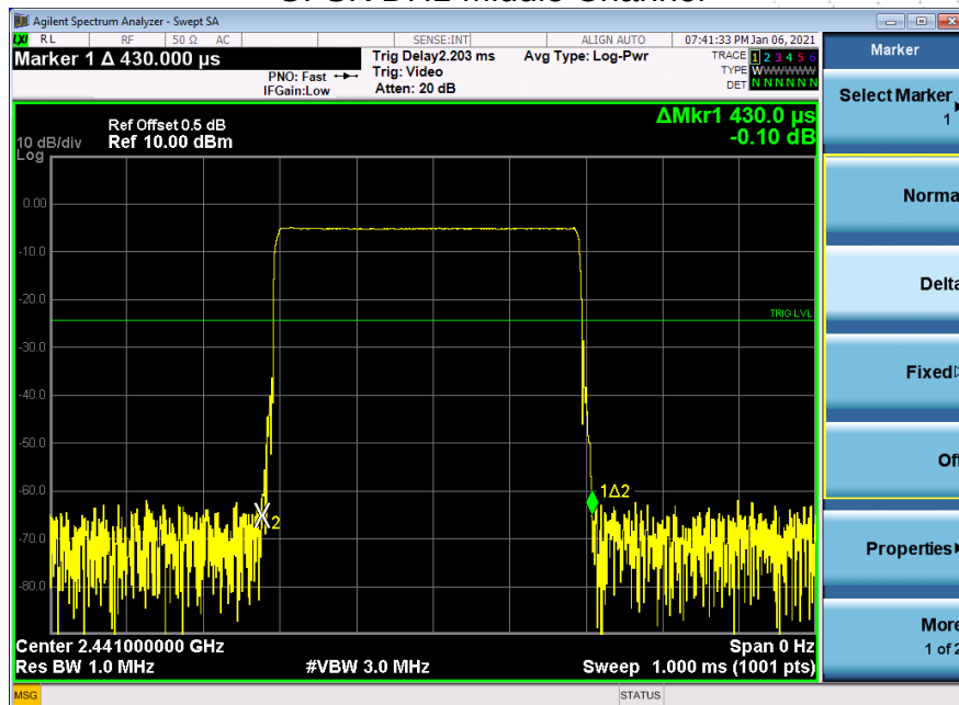
Test Plots GFSK DH1 Middle Channel
