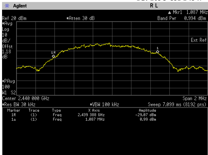
Frequency 2440 MHz
