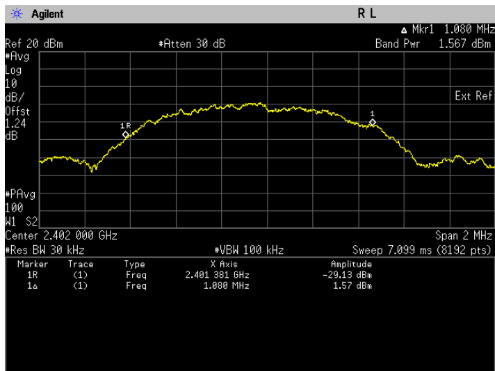
Frequency 2402 MHz
