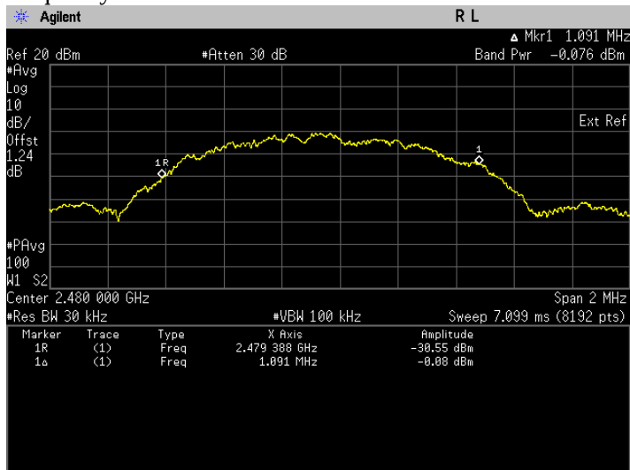
Frequency 2480 MHz
