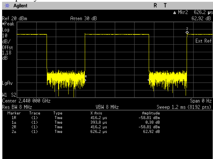
Duty Cycle
