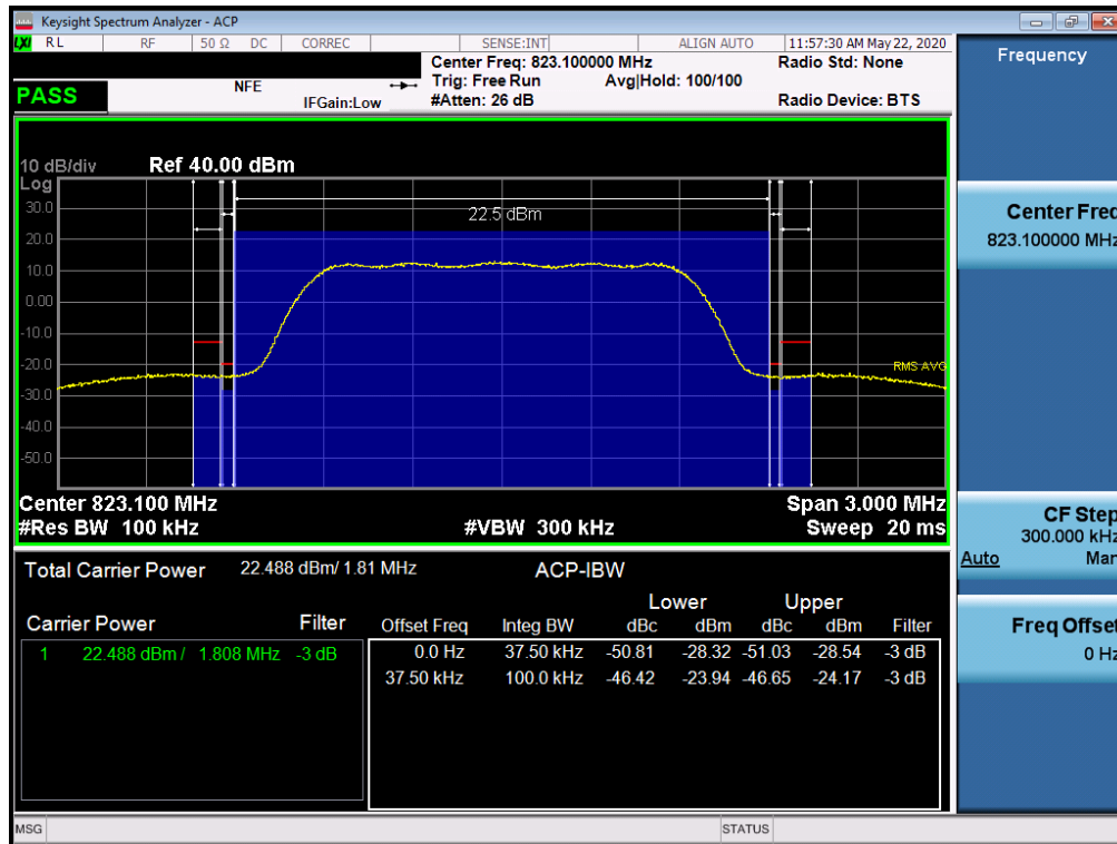
Plot 7-30. Channel Edge Plot (CDMA BC10 – Ch. 684)
