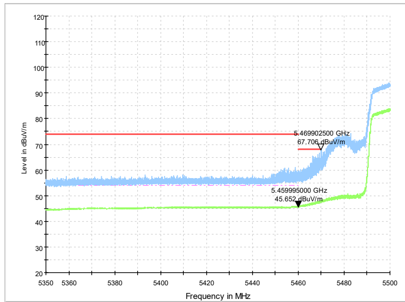
Fig. 11 Band Edges (802.11n-HT40 Ch102, 5510MHz)
