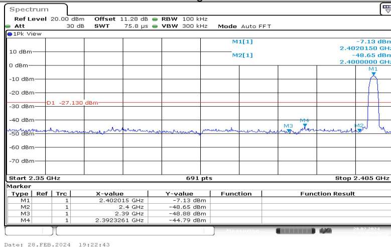
2DH5-Ant1-Low-2402--7.13
