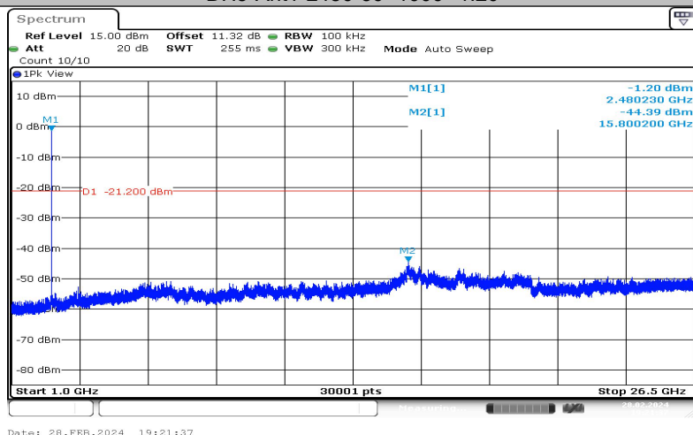
DH5-Ant1-2480-1000~26500--1.20
