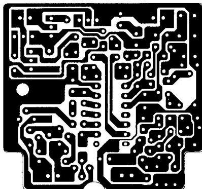
PCB NO. 9639-21 SOLDER SIDE
