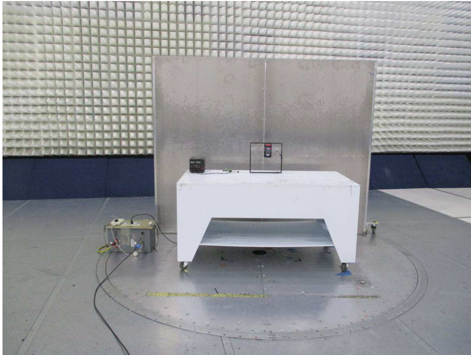
AC line conducted emission test
